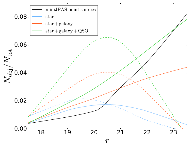
Figure 2. Original (dashed lines) and shifted (solid coloured lines) SDSS r -band magnitude distributions of a sample containing equal numbers of stars, galaxies, and quasars ( 10^4 of each). As a comparison, the black solid line shows the magnitude distribution of miniJPAS point-like sources. The y-axis corresponds to the number of objects in each magnitude bin divided by the total number of objects in the corresponding sample. The total number of objects are 10k, 20k, 30k, and 11 419 for the green, orange, blue, and black curves, respectively.
