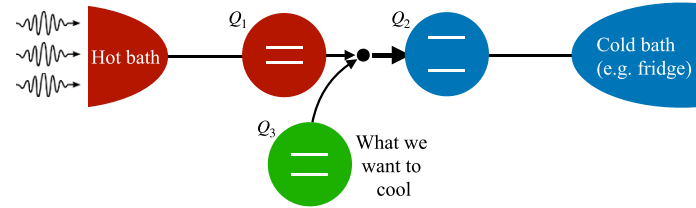
Figure 5. Schematics of a quantum absorption refrigerator with 3 qubits. Heat naturally flows from the hot bath to the cold bath, through qubits Q_1 and Q_2 . However, the qubits' frequencies \omega_{1/2} are designed to be far off-resonance blocking the natural flow. A third qubit Q_3 is introduced with a gap \omega_3 , designed so that \omega_1 + \omega_3 = \omega_2 . This resonance condition allows for two excitations, one in Q_1 and one in Q_3 , to be converted into a single excitation in Q_2 . Any excitation in Q_3 will therefore be sucked off by the hot/cold temperature gradient. The device therefore operates like an autonomous refrigerator helping qubit Q_3 cool.
