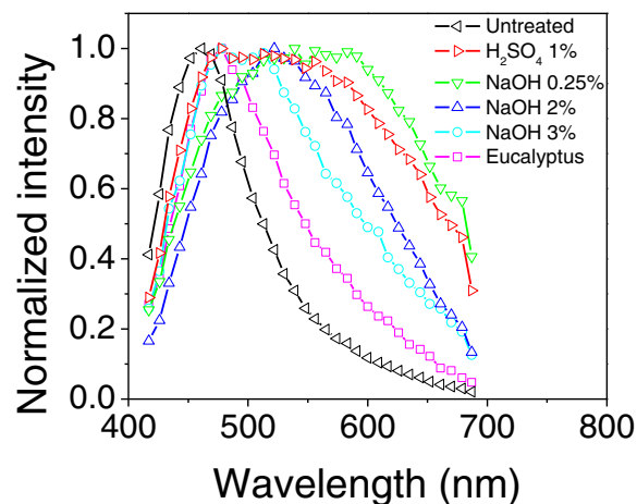
Figure 5 Fluorescence spectra for two-photon excitation.
