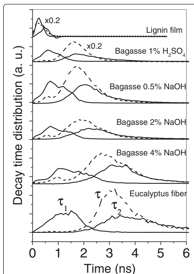
Figure 3 Effect of NaOH treatment on the decay time distribution. Rapid ( \tau_1 ) and slow ( \tau_2 ) decay time distributions evaluated from FLIM image and the corresponding average decay time ( \tau ) for bagasse treated with H 2 SO 4 1%, NaOH 0.5%, 2% and 4%. The same distributions are also presented for the eucalyptus fiber and the lignin film for comparison. The factor 0.2 was used just to set the counts to a convenient value just to get a better comparison among distributions.
