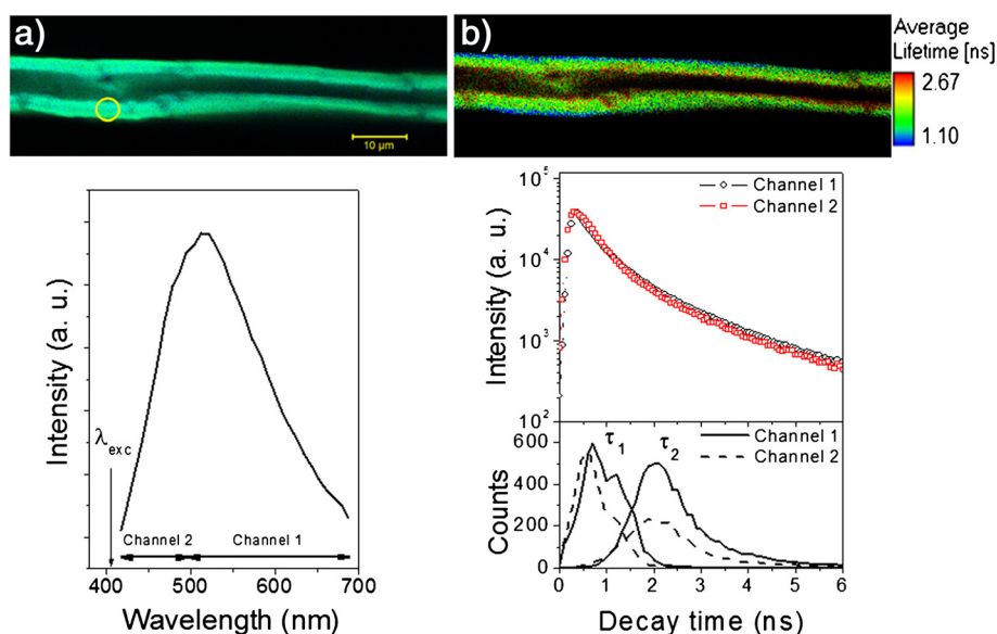
Figure 1 Confocal and FLIM images for a single bagasse fiber: spectral and fluorescence decay features. a) Spectral confocal image of a single bagasse fiber treated with NaOH 0.5% excited at \lambda_{exc} = 405 nm (continuous wave). The spectrum below corresponds to the emission evaluated at the yellow spot of the cell wall. The spectral regions for channels 1 and 2 used in the decay time measurements are displayed in the figure. b) The corresponding FLIM image and the associated decay features detected from channels 1 and 2. The figure below shows the decay time distributions for \tau_1 and \tau_2 evaluated from the FLIM image for channel 1 (solid lines) and channel 2 (dashed lines).
