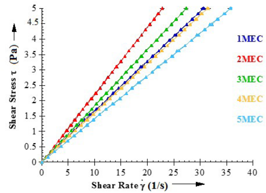
Figure 1. Flow curves of the developed MECs containing ethanolic extract of C. glabrata at 25 °C.
