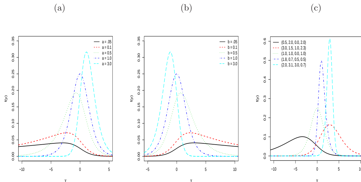
Figure 5: Plots of the KumL density function for some parameter values. (a) For b = 1 , \mu = 0 and \sigma = 1 . (b) For a = 1 , \mu = 0 and \sigma = 1 . (c) For values different of a , b , \mu and \sigma .
