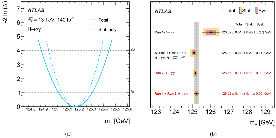
Fig. 3. (a) Value of -2\ln\Lambda as a function of m_H for the combined fit to all H \rightarrow \gamma\gamma categories. The intersections of the -2\ln\Lambda curve with the horizontal lines labelled 1\sigma and 2\sigma provide the 68.3% and 95.5% confidence intervals. (b) Summary of the Higgs boson mass measurements from the analysis of H \rightarrow \gamma\gamma decays in ATLAS Run 2 data and combined Run 1 + Run 2 data presented in this Letter, compared with the combined Run 1 ATLAS result in the diphoton channel and with the Run 1 measurement by ATLAS and CMS [9] combining the diphoton and four-lepton channels. The statistical, systematic and total uncertainties are indicated with horizontal yellow-shaded bands, pink-shaded bands and black error bars, respectively. The vertical dashed line and grey shaded band around it indicate the central value and total uncertainty of the H \rightarrow \gamma\gamma ATLAS Run 1 + Run 2 measurement.
