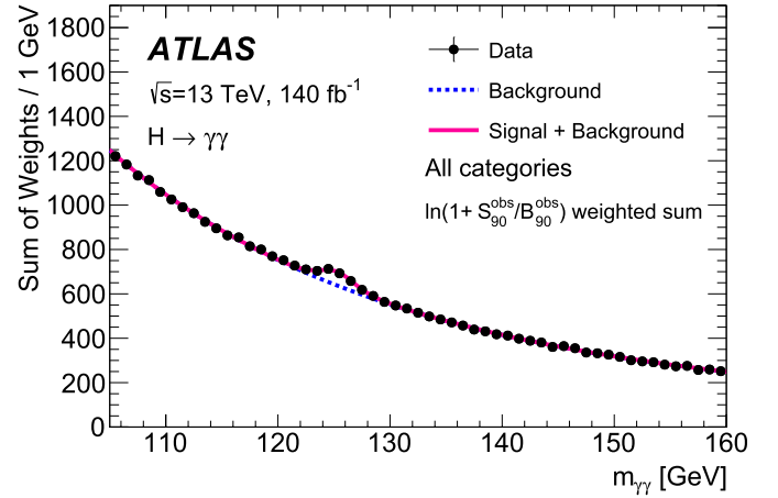
Fig. 2. Diphoton invariant mass distribution of all selected data events (black dots with error bars), overlaid with the result of the fit (solid red line). For both the data and the fit, each category is weighted by a factor \ln(1 + S_{90}^{\text{obs}}/B_{90}^{\text{obs}}) , where S_{90}^{\text{obs}} and B_{90}^{\text{obs}} are the fitted signal and background yields in the smallest m_{\gamma\gamma} interval containing 90% of the expected signal. The dotted line describes the background component of the model.
