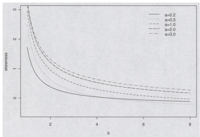
Figure 6 Skewness of the BBIII distribution as a function of b for some values of a and \alpha = 5 , \beta = 2 and s = 1 .
