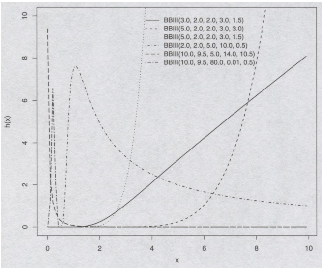
Figure 5 Plots of the BBIII hazard rate function.
