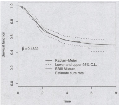
Figure 15 Estimated survival function for the BBIII mixture model and the empirical survival for melanoma data.
