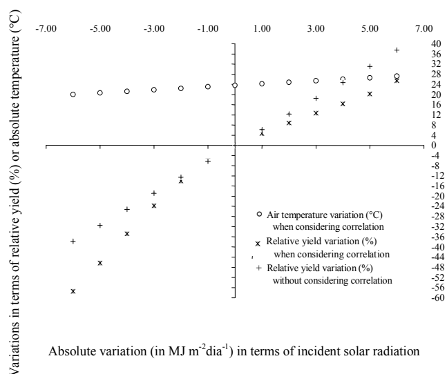
Figure 3. Sensitivity analysis for the absolute variation in temperature and relative yield from each unit of MJ m^{-2} d^{-1} varied in terms of incident solar radiation.
