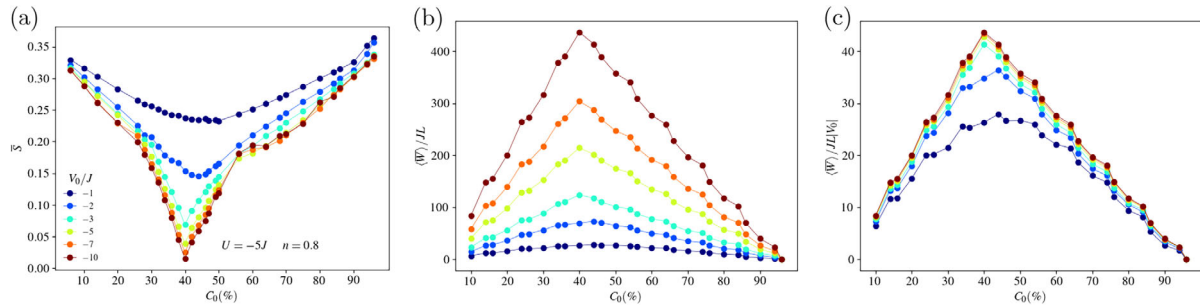
Figure 2. Panel a): Single-site entanglement averaged over 100 of the possible impurity configurations versus concentration. Panel b): \overline{\langle W \rangle}/(JL) , averaged over 100 of the possible impurity configurations, versus initial concentration Panel c): Average work from panel (b) scaled by the disorder strength |V_0| .
