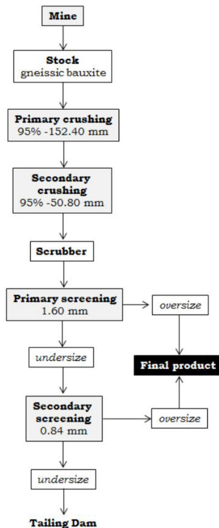
Figure 1. Simplified Mirai plant flowsheet.
