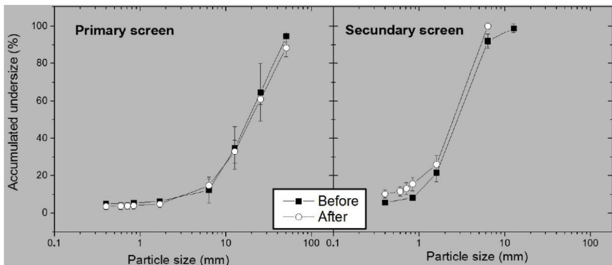
Figure 6. Particle size distributions for primary and secondary screens before and after the project.
