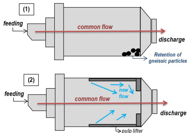
Figure 3. Unloader system installed into the scrubber.
