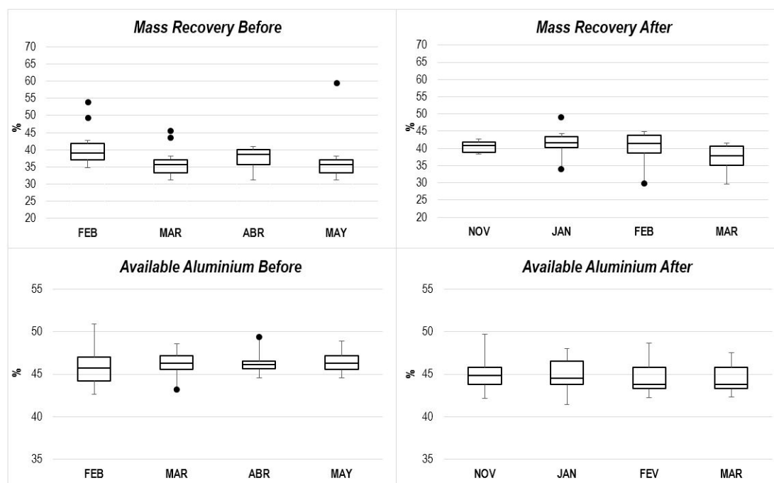
Figure 5. Boxplots of mass recovery and available aluminium (AA) content before and after the operation modifications.
