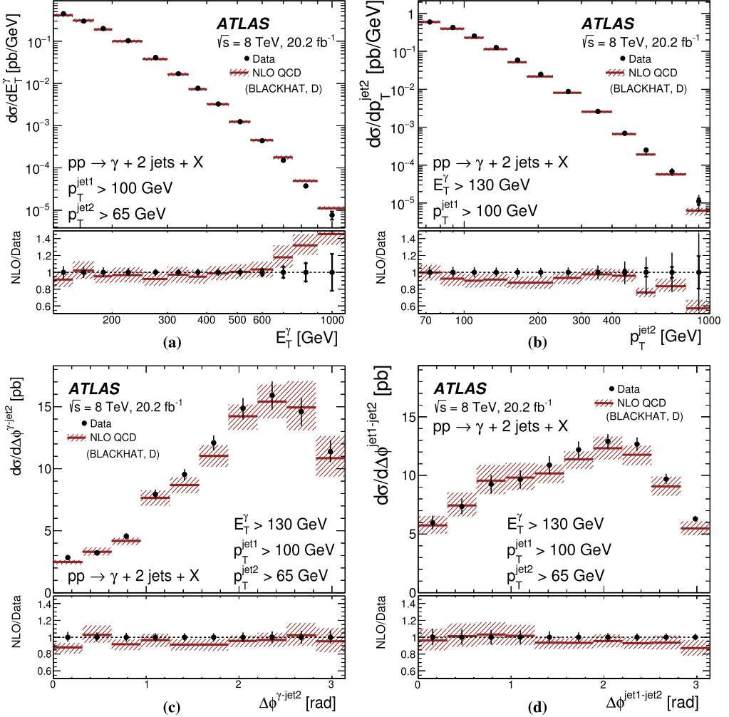
Fig. 8. Measured cross sections for isolated-photon plus two-jet production (dots) as functions of (a) E_T^\gamma , (b) p_T^{\text{jet2}} , (c) \Delta\phi^{\gamma\text{--jet2}} and (d) \Delta\phi^{\text{jet1--jet2}} . The NLO QCD predictions from BLACKHAT corrected for hadronisation and underlying-event effects and using the CT10 PDF set (solid lines) are also shown. These predictions include only the direct contribution (D). The bottom part of each figure shows the ratio of the NLO QCD prediction to the measured cross section. The inner (outer) error bars represent the statistical uncertainties (the statistical and systematic uncertainties added in quadrature) and the shaded band represents the theoretical uncertainty. For most of the points, the inner error bars are smaller than the marker size and, thus, not visible.
