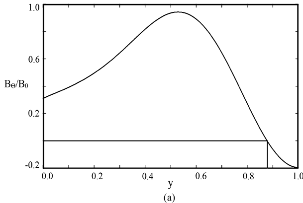
Fig. 3. (a) Poloidal magnetic field profile, which is null at y = 0.876 ; (b) Safety factor profile, with a divergence in y = 0.876 .
