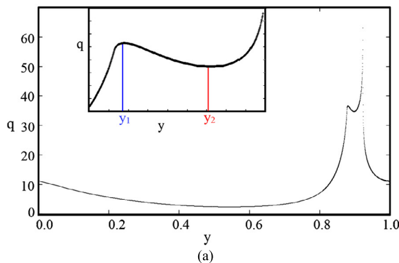
Fig. 4. (a) Numerical safety factor profile. We fixed x = 0.51 to obtain this profile. In the inset, we highlight the maximum and minimum points; (b) Shearless line and island chains.
