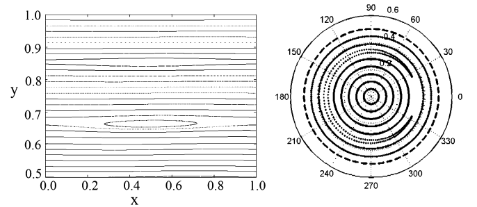
Fig. 9. Regular magnetic surfaces for the original Tokamap with L = 0.05 .
