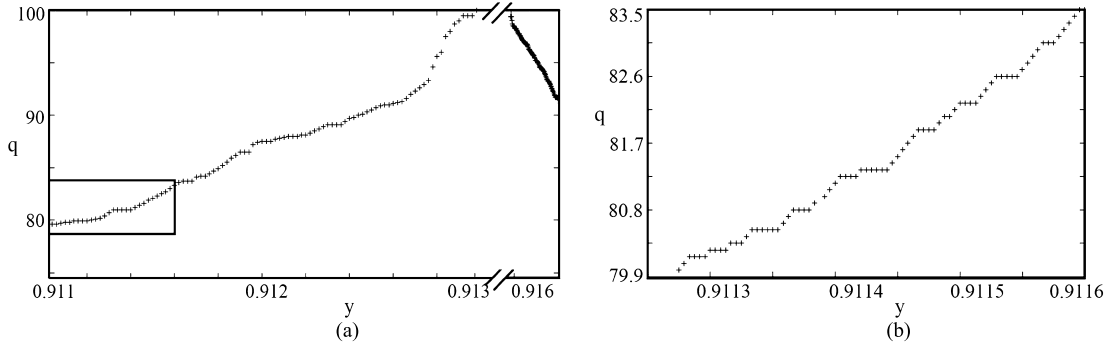
Fig. 8. (a) Numerical safety factor profile. (b) Amplification of the profile box showing the levels when the values are constant, indicating the presence of the islands.
