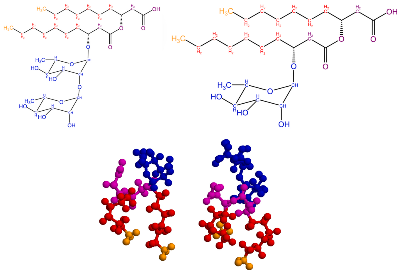
Fig. 1. Structure (top) and ball-and-stick representation (bottom) of mono-RL (left) and di-RL (right). Red, orange, magenta, and blue, correspond to \text{CH}_2 , \text{CH}_3 , the negatively charged CR ( (\text{CH})(\text{CH}_2)(\text{COO})(\text{CH})(\text{CH}_2)(\text{COO}^-) ), the rhamnose group RHA ( \text{O}(\text{CHO})(\text{CHCH}_3)(\text{CHOH})_3 ) or the rhamnose-rhamnose group RHA-RHA ( \text{O}(\text{CHO})(\text{CHCH}_3)(\text{CHOH})_2(\text{CH})_2(\text{OH}) ).
