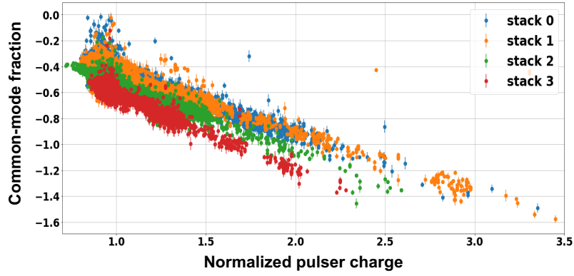
Figure 8. The common-mode fraction ( k_{\text{CF,pad}} ) as a function of normalized pulser charge ( Q_{\text{pulser,pad}}^{\text{norm}} ) for each stack, only for the data with uncertainty of k_{\text{CF,pad}} less than 5%.
