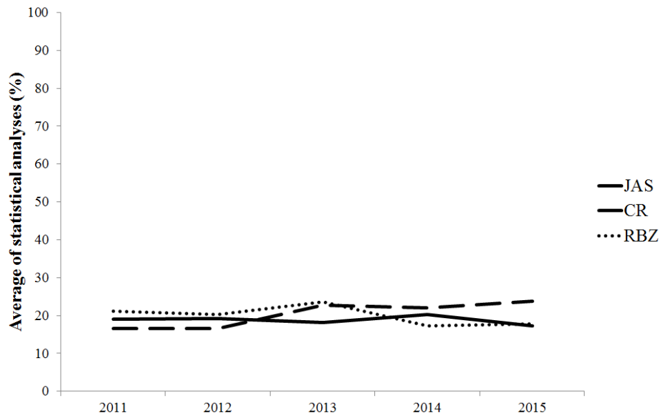
Figure 5 - Graph of average profiles for statistical analyses used as a percentage for each journal in each year of the period studied. JAS – Journal of Animal Science; CR – Ciência Rural; RBZ – Revista Brasileira de Zootecnia.
