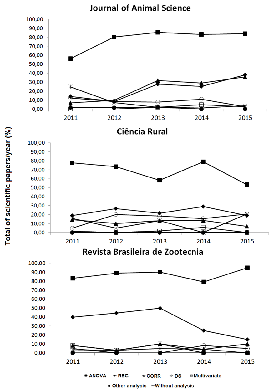
Figure 4 - Statistical analyses used over the years in scientific papers published on JAS, CR and RBZ during the period from 2011 to 2015. ANOVA - Analysis of variance and mean comparison; REG - Regression analysis; CORR - Correlation analysis; DS - Descriptive statistics.
