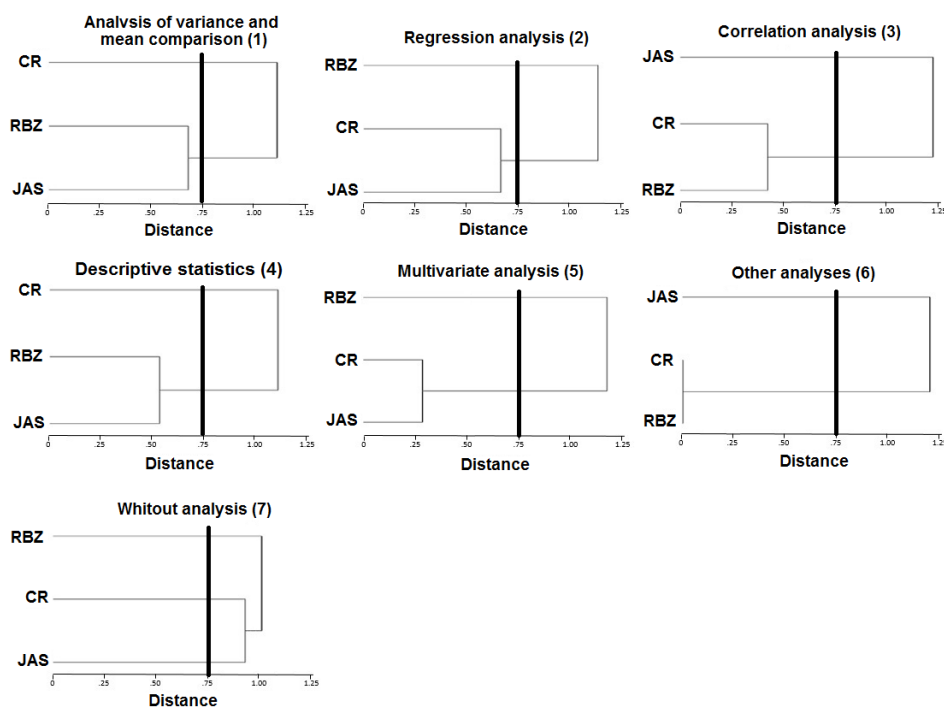
Figure 1 - Cluster analysis among journals for each statistical analysis. JAS – Journal of Animal Science; CR – Ciência Rural; RBZ – Revista Brasileira de Zootecnia.
