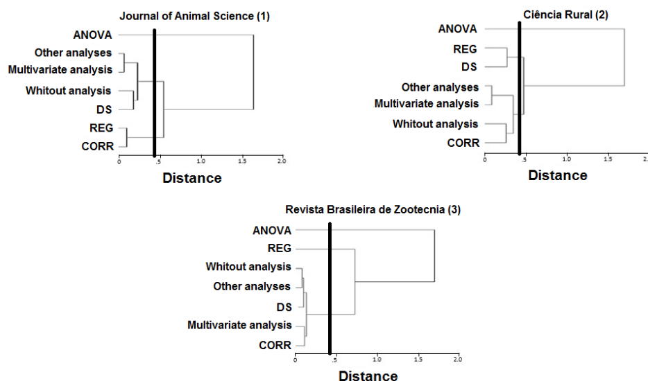
Figure 2 - Cluster analysis between statistical analyses used for each journal. ANOVA - Analysis of variance and mean comparison; REG - Regression analysis; CORR - Correlation analysis; DS - Descriptive and graphic statistics.
