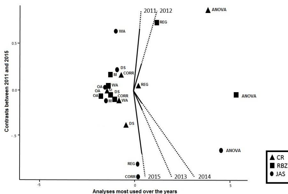
Figure 3 - Biplot graphic for principal components analysis on statistical analyses for each journal, according to the years studied. ● = JAS (Journal of Animal Science); ▲ = CR (Ciência Rural); ■ = RBZ (Revista Brasileira de Zootecnia); ANOVA - Analysis of variance and mean comparison; REG - Regression analysis; CORR - Correlation analysis; DS - Descriptive statistics; M - Multivariate analysis; OA - Other analyses; WA - without analysis.
