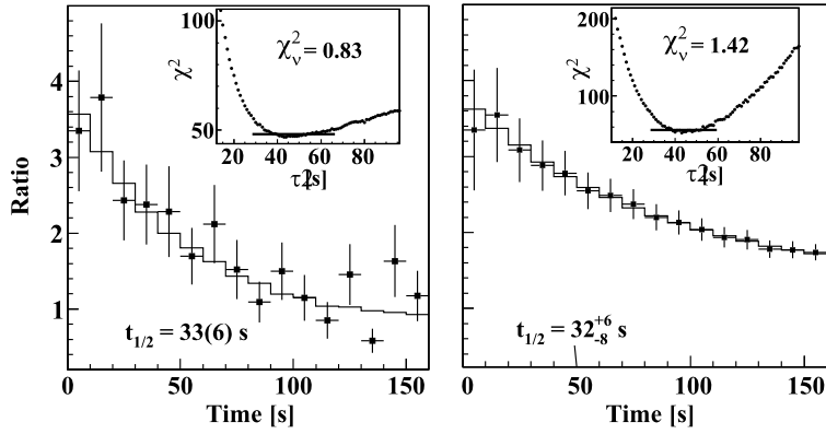
Fig. 2. Experimentally (symbols) and numerically (solid lines) determined ratios between forward and backward time distributions for ^{218}\text{Bi} sorted in standard and accumulated format (left and right panel). In the insets the \chi^2 minimization for the distributions are shown. (See text for details).
