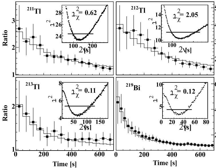
Fig. 3. Experimentally (symbols) and numerically (solid lines) determined ratios between forward and backward distributions for ^{211,212,213}\text{Tl} and ^{219}\text{Bi} , together with the \chi^2 minimization in the insets. Resulting half-lives are given in the text.
