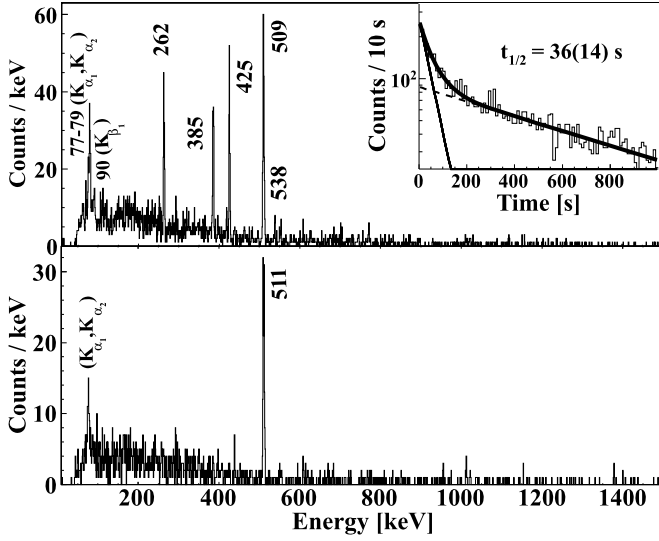
Fig. 1. \gamma spectra correlated with the \beta decay of ^{218}\text{Bi} . In the top panel the correlations are performed in standard time sequence showing the expected \gamma -ray transitions from the known decay scheme [14] together with characteristic X rays. The bottom panel shows correlations performed in time reversal order to highlight random correlations. The inset in the panel shows the time distribution obtained in coincidence with the 262-, 385- and 425-keV transitions together with the analytical fit by a double component exponential-decay function, in order to account for the background.
