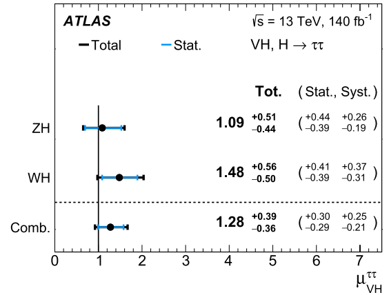
Fig. 4. The fitted values of the Higgs boson signal strength \mu_{VH}^{\tau\tau} for m_H = 125 GeV for the WH and ZH processes and their combination from the NN-based fit. The individual \mu_{VH}^{\tau\tau} values for the (W/Z)H processes are obtained from a simultaneous fit with the signal strength for each of the WH and ZH processes floating independently. The probability of compatibility of the individual signal strengths is 56%.
