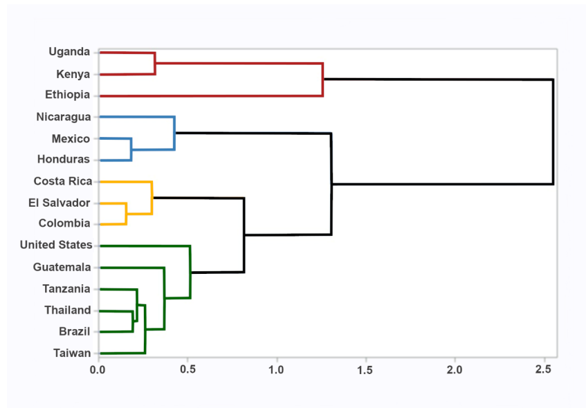
Figure 2: Cluster analysis of coffee quality attributes from 15 producing countries.
