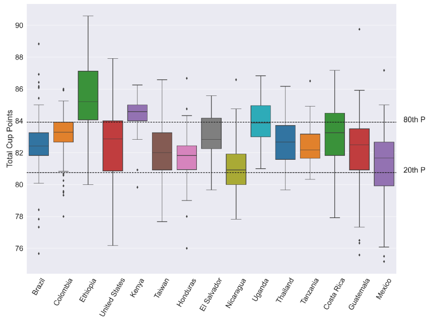
Figure 3: Boxplots of total cup points with percentiles for 15 producing countries.
