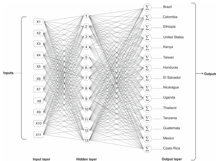
Figure 1: Network architecture used in the Multilayer Perceptron.
