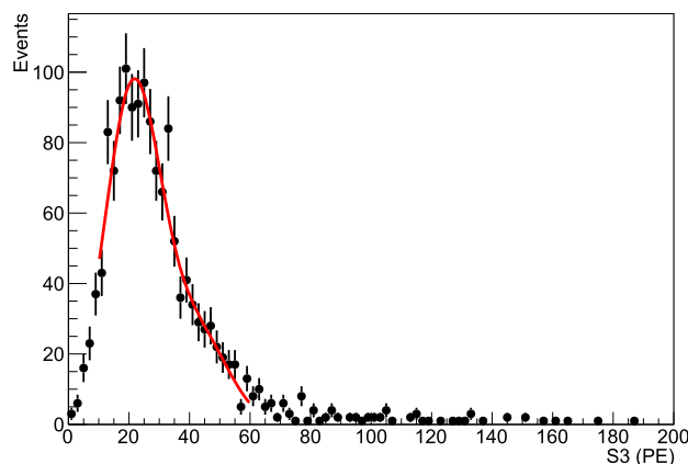
Right: S3 charge distribution for events in which the delay between S2 and S3 signals is within (T_{max} \pm 4) \mu\text{s} , superimposed with the fit described in the text
