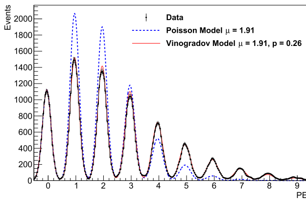
Fig. 6 A typical charge distribution, in number of photoelectrons, for a bottom channel (black histogram), superimposed with a pure Poisson model with \mu = 1.91 (blue dashed line) and a compound Poisson model of Eq. 1 with \mu = 1.91 and p = 0.26 (red solid line)
