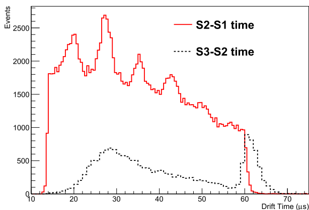
Fig. 19 Left: Distribution of the drift time between S1 and S2 signals (red curve) and between S2 and S3 signals (black curve) for a set of ^{241}\text{Am} measurements taken in double-phase mode at \mathcal{E}_d = 183 \text{ V/cm} .
