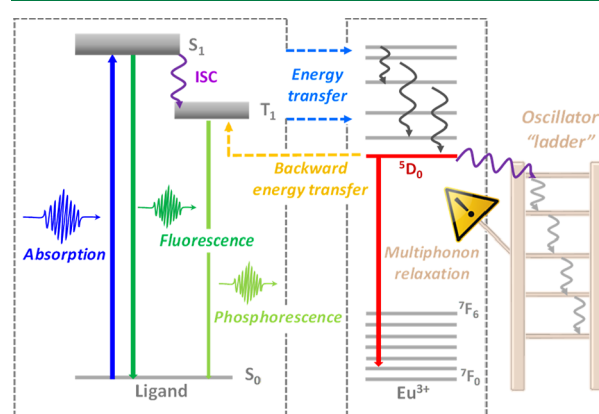
Figure 3. Multiphonon relaxation scheme in an \text{Eu}^{3+} complex where the oscillator ladder can be seen as the acceptor vibrational mode.
