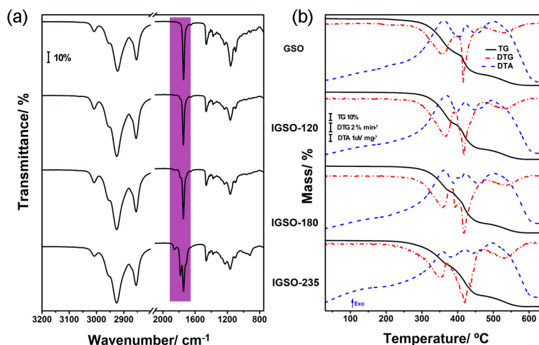
Figure 10. (a) MIR-ATR spectra and (b) TG/DTG-DTA curves obtained for GSO (grape seed oil) and the IGSO (itaconized grape seed oil) samples obtained at different temperatures: 120 °C (IGSO-120), 180 °C (IGSO-180), and 235 °C (IGSO-235) under microwave irradiation.
