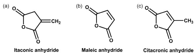
Figure 1. Chemical structures of different anhydrides: (a) ITA, (b) MA and (c) CTA.
