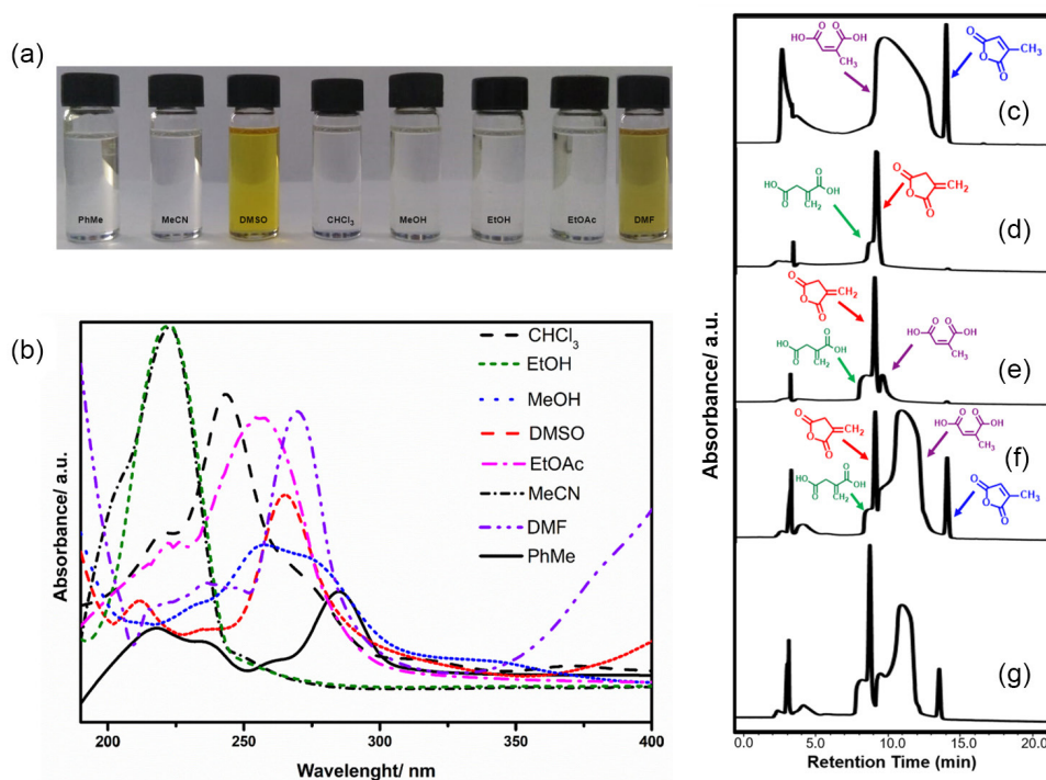
Figure 6. (a) ITA (itaconic anhydride) solubilized in different organic solvents, (b) UV spectra of ITA in different organic solvents (1 mmol L -1 ), and HPLC-DAD chromatograms obtained for samples, (c) CTA (citraconic anhydride), (d) ITA, (e) ITA heated to 150 °C, and ITA heated to 250 °C, (f) non-volatile sample and (g) volatile sample.
