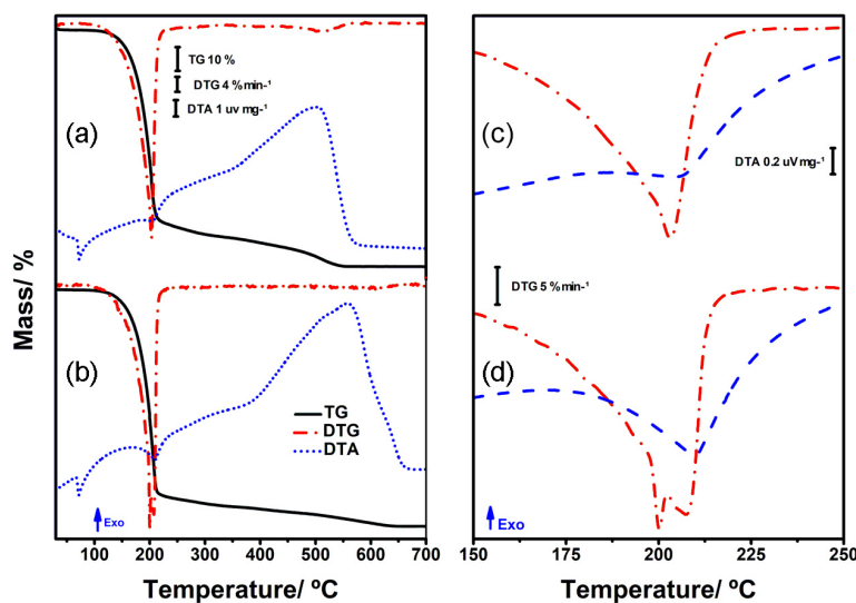
Figure 3. TG/DTG-DTA curves of ITA (itaconic anhydride) in (a) dry air atmosphere, (b) \text{N}_2 atmosphere as well as magnification between 150 and 250^\circ\text{C} under (c) air atmosphere, and (d) \text{N}_2 atmosphere.
