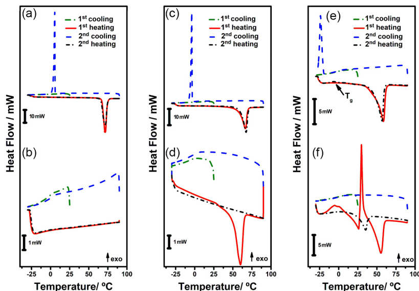
Figure 7. DSC curves of (a) ITA (itaconic anhydride), (b) CTA (citraconic anhydride), (c) ITA heated to 150 °C, (d) ITA heated to 210 °C, and ITA heated to 250 °C, (e) liquid sample and (f) solid sample (copolymer).
