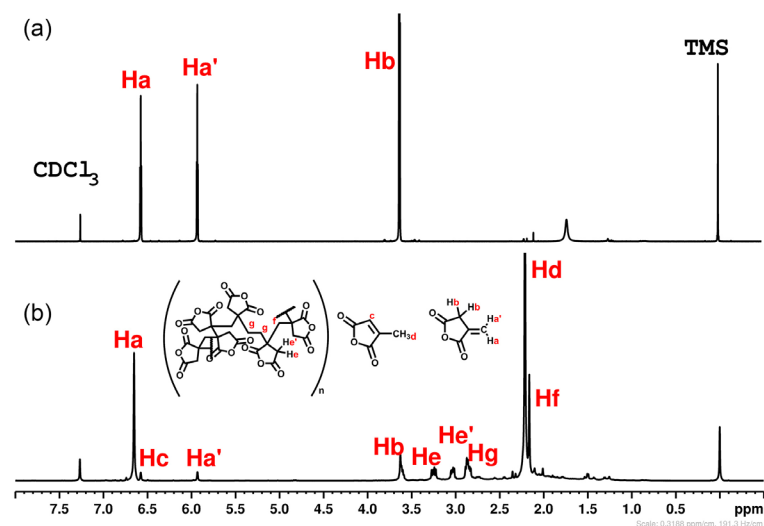
Figure 5. ^1\text{H} NMR spectra (600 MHz, \text{CDCl}_3 ) of ITA (itaconic anhydride) at (a) 25 °C and (b) heated to 230 °C in TG-DTA system.
