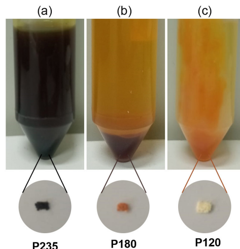
Figure 2. Reaction mediums obtained after itaconic anhydride incorporation into grape seed oil by microwave irradiation in different temperatures, as well as the precipitated obtained in each synthesis: (a) 235^\circ\text{C} , (b) 180^\circ\text{C} , and (c) 120^\circ\text{C} .
