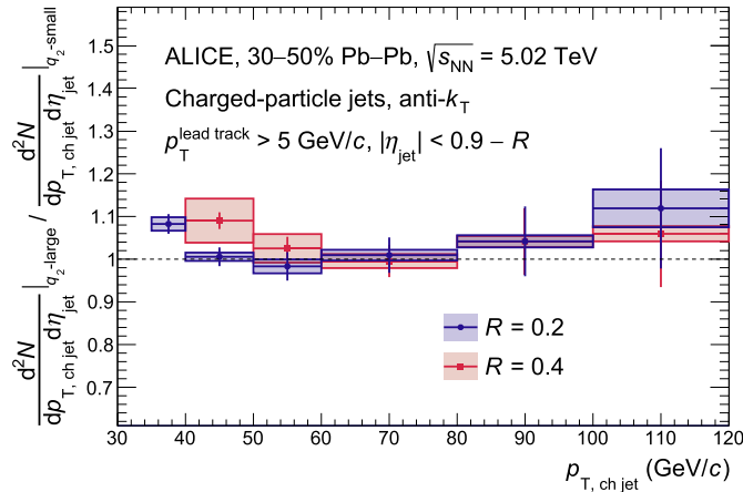
Fig. 3. Ratio of the charged-particle jet yields of the q_2 -large to the q_2 -small event classes, in Pb-Pb collisions at \sqrt{s_{NN}} = 5.02 TeV. The results are reported for R = 0.2 and R = 0.4 jets.
