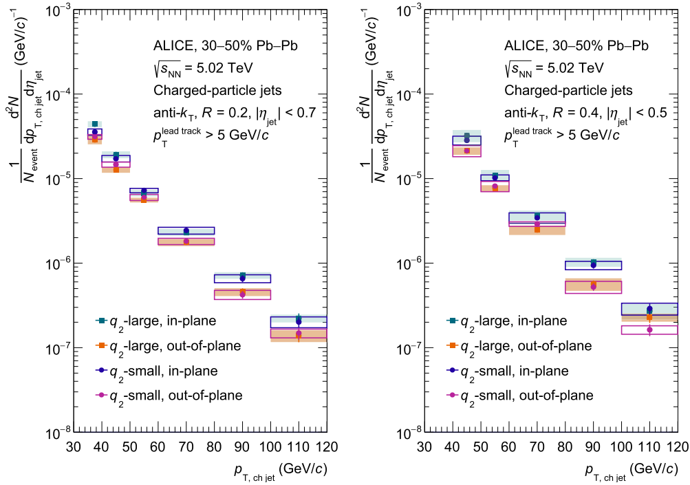
Fig. 2. Charged-particle jet yields for R = 0.2 (left) and R = 0.4 (right) jets in Pb-Pb collisions at \sqrt{s_{NN}} = 5.02 TeV. Results are shown for the q_2 -small and q_2 -large event classes, for in- and out-of-plane jets. The bars (boxes) represent statistical (systematic) point-by-point uncertainties.
