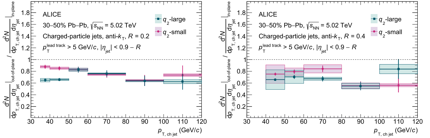
Fig. 4. Ratios of out-of-plane to in-plane charged-particle jet yields for the q_2 -large and q_2 -small event classes in Pb-Pb collisions at \sqrt{s_{NN}} = 5.02 TeV. The results are reported for R = 0.2 (left) and R = 0.4 (right) jets, and are corrected for the event-plane resolution.
