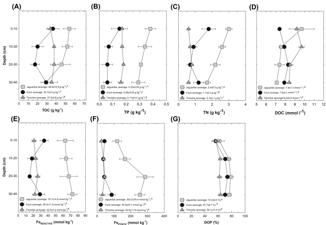
Fig. 4. Contents of total organic carbon (TOC; A), total phosphorus (TP; B), total nitrogen (TN; C), dissolved organic carbon (DOC; D), reactive and pyritic Fe (Fe REACTIVE and Fe PYRITE ; E and F, respectively) and degree of pyritization (DOP) for the three mangroves (Timonha River, control site; Cocó River, affected by urban wastes; and Jaguaribe River, affected by shrimp farming). The average values followed by different capital letters present significant different values ( P < 0.005 ).
