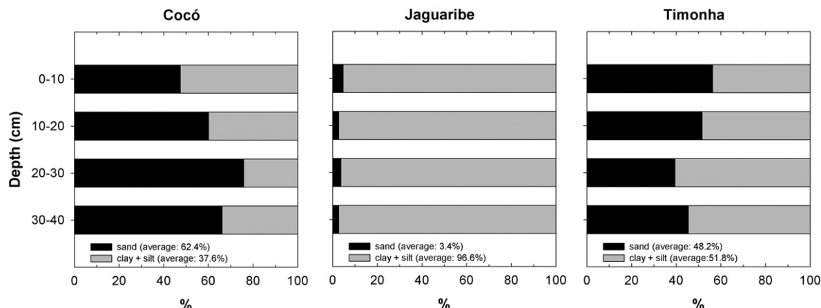
Fig. 3. Sand and silt + clay contents for the three mangroves (Timonha River, control site; Cocó River, affected by urban wastes; and Jaguaribe River, affected by shrimp farming).
