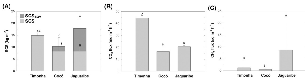
Fig. 5. Soil carbon stock (A) CO 2 (B) and CH 4 (C) fluxes from the different mangroves (Timonha River, control site; Cocó River, affected by urban wastes; and Jaguaribe River, affected by shrimp farming). For the SCS, CO 2 and CH 4 fluxes, the averages values followed by different capital letters present significant different values ( P < 0.005 ). For the SCS EQV , the averages values followed by different lowercase letters present significant different values ( P < 0.005 ).
