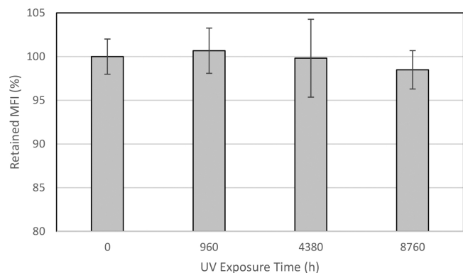
Figure 1. Retained MFI test results compared with virgin sample test result after UV fluorescent exposure
