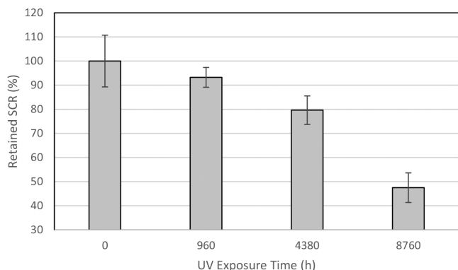
Figure 3. Retained SCR test results compared with virgin sample test result after UV fluorescent exposure
