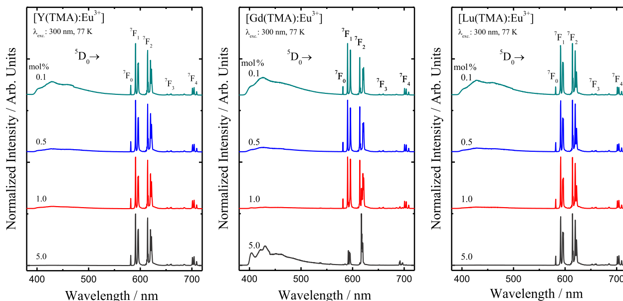
Fig. 5. Emission spectra of the doped [RE(TMA):Eu^{3+}(x \text{ mol\%})] systems recorded at 77 K, under excitation at 300 nm.
