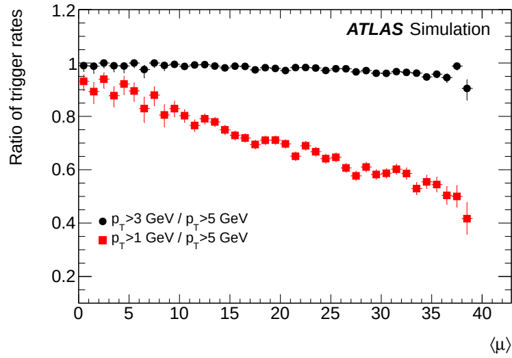
Figure 16. Ratio of trigger rates as a function of \langle\mu\rangle when using lower p_T isolation cuts for the Muon RoI Cluster trigger compared to the p_T > 5 \text{ GeV} cut used online.
