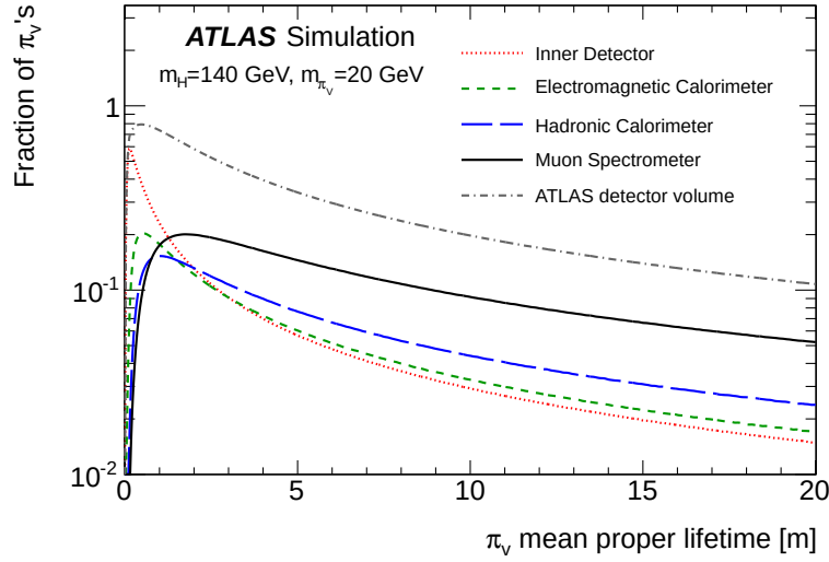
Figure 1. The probability of a \pi_v to decay in the ID (beyond the second layer of the pixel detector), ECal, HCal, MS and the whole ATLAS detector as a function of the \pi_v mean proper lifetime ( c\tau ) for |\eta| < 2.5 . The sample with m_H = 140 GeV and m_{\pi_v} = 20 GeV is used.
