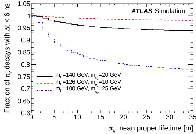
Figure 10. Fraction of \pi_v decays producing a Muon RoI Cluster trigger associated with the correct bunch crossing as a function of the \pi_v mean proper lifetime.
