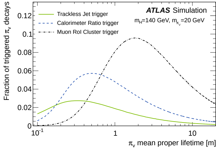
Figure 14. The expected fraction of events that pass each of the long-lived neutral particle triggers as a function of the \pi_\nu mean proper lifetime.
