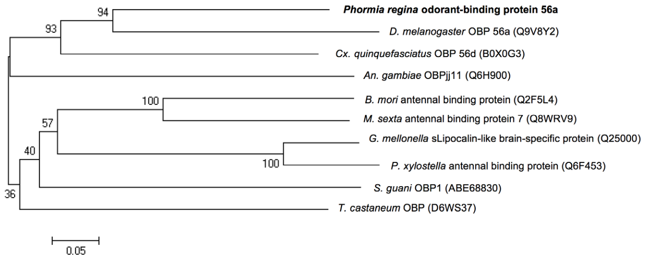
Figure 2. Nucleotide and deduced amino acid sequences and phylogenetic analysis of oral disk-specific protein (PregOBP56a). A, cDNA and deduced amino acid sequences of an oral disk-specific protein. A signal peptide is shown in italic. N-terminal amino acid sequence determined by Edman degradation is underlined. Arrowheads show 6 cysteine residues, which are hallmarks of insect classic OBPs. The three arrows indicate annealing sites of a degenerate (EEQKAKV-1) and two gene-specific (PregOBP56a-1 and PregOBP56a-2) primers. B, Phylogenetic tree of odorant-binding protein 56a like-protein sequences. Phormia regina odorant-binding protein 56a is shown in bold. Accession numbers of each protein are given in the parenthesis. Bootstrap values were determined from 1,000 replications. Bar indicates 5% divergence. doi:10.1371/journal.pone.0051779.g002
