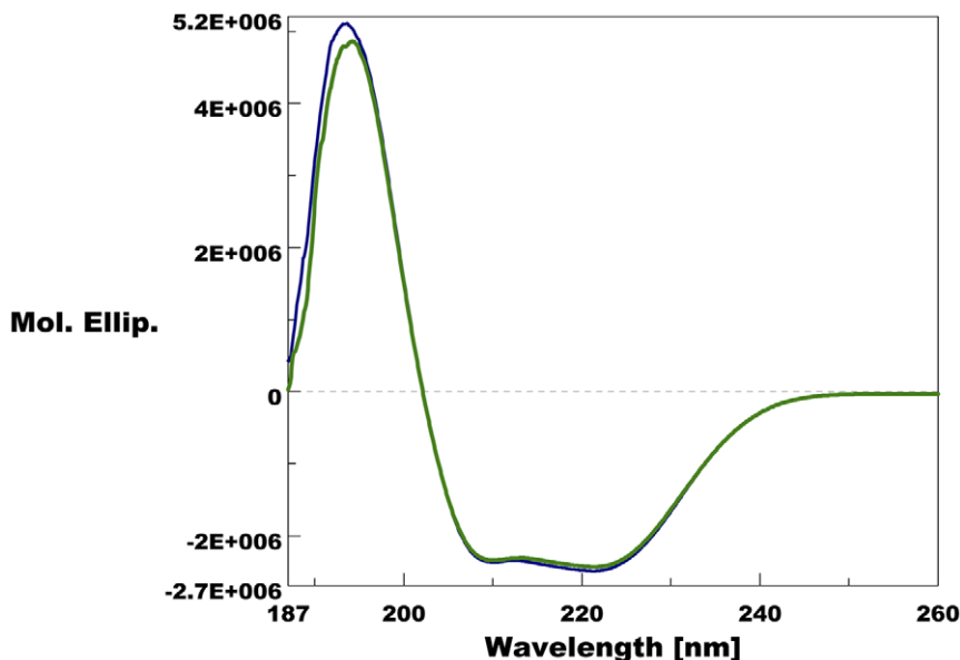
Figure 4. Far UV circular dichroism spectra of purified recombinant PregOBP56a . A positive peak of the CD spectra at 194 nm and two negative peaks at 209 and 221 nm are observed at pH 7 and pH 5, indicating that PregOBP56a is an \alpha -helix-rich protein as other insect OBPs. doi:10.1371/journal.pone.0051779.g004
