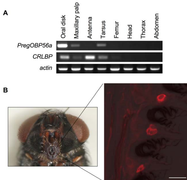
Figure 3. Expression of PregOBP56a . A, Tissue specificity of PregOBP56a expression. cDNA was synthesized from total RNA extracted from each experimental tissue at day 0 adult stage. Gene expression was detected by RT-PCR. actin expression was used as an internal control. PregOBP56a was highly expressed in the oral disk. In contrast CRLBP , an OBP related to chemical reception, was expressed in the oral disk and antenna. B, Cellular localization of PregOBP56a expression in the oral disk by in situ hybridization. Sense and anti-sense probes were prepared by pSTP18 inserted with a PCR product amplified by primers PregOBP56a -1 and PregOBP56a -2. The left panel shows the localization of the oral disk within the head of a female. The right panel shows the localization of PregOBP56a transcripts in a cluster of cells that are localized between pseudotracheae. Scale bar is 20 \mu m. doi:10.1371/journal.pone.0051779.g003
