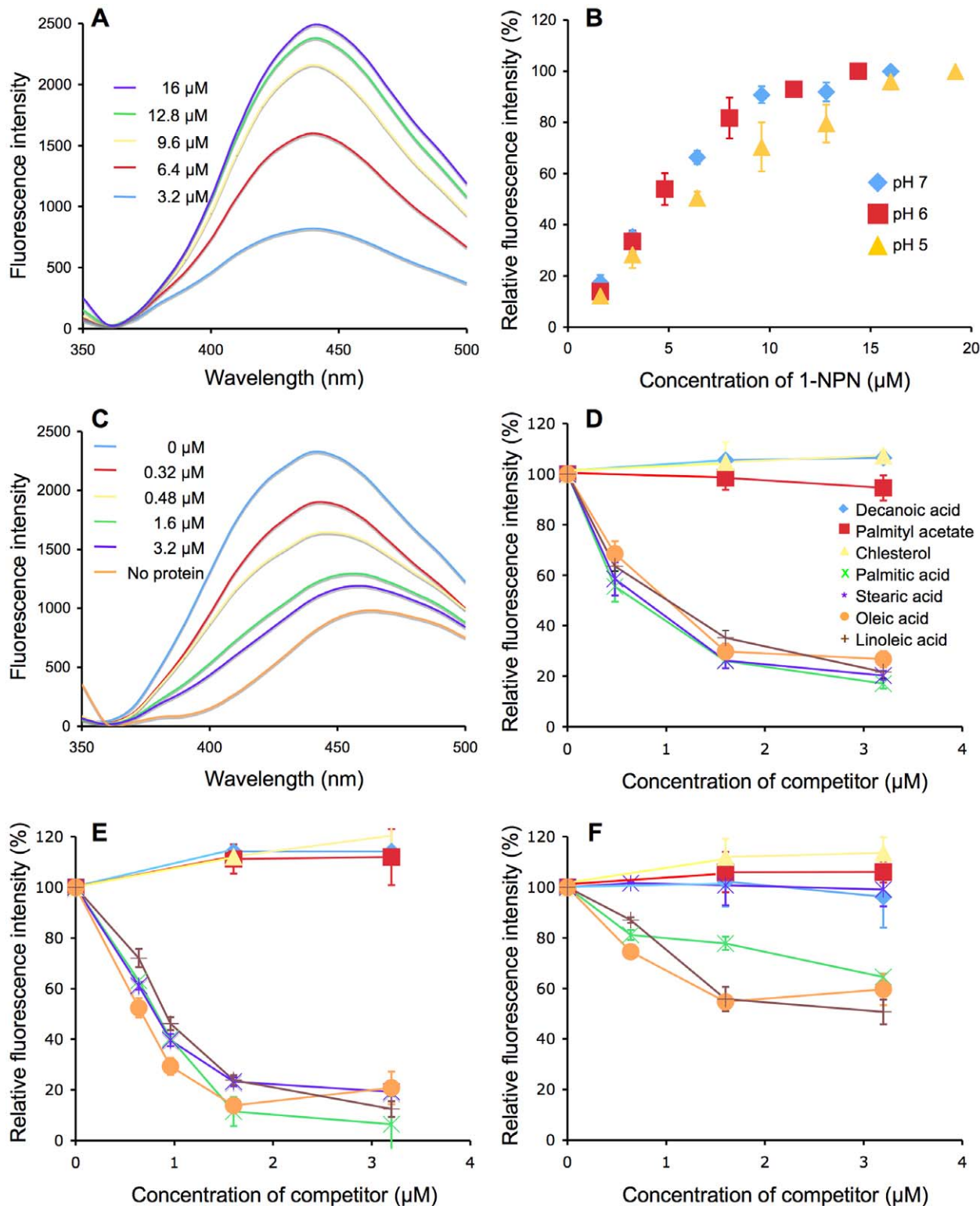
Figure 5. Binding of PregOBP56a to N -phenyl-1-naphthylamine (1-NPN) and potential ligands derived from chicken meat. A, A typical emission spectra following the addition of 1-NPN (3.2–16 \mu\text{M} final concentration) to recombinant PregOBP56a (10 \mu\text{g}/\text{ml} of 20 mM phosphate-citrate buffer, pH 7). The emission spectra were generated following excitation at a wavelength of 337 nm. B, Binding of 1-NPN to PregOBP56a at pH 7, 6, and 5. In these experiments PregOBP56a (10 \mu\text{g}/\text{ml} ) was incubated with various concentrations (1.6–19.2 \mu\text{M} ) of 1-NPN and emission at 440 nm was plotted. Values are means \pm standard deviation, n=3 . C, Typical emission spectra following the addition of a competitor to PregOBP56a bound to 1-NPN. PregOBP56a (10 \mu\text{g}/\text{ml} ) in 20 mM phosphate-citrate buffer at pH 7 was pre-incubated with 16 \mu\text{M} of 1-NPN (final concentration). Then, palmitic acid (0–3.2 \mu\text{M} final concentration) was added to the reaction, and the emission spectra (excitation a wavelength of 337 nm) were recorded. D, Binding of PregOBP56a to various ligands at pH 7. For each set of data, fluorescence values at a wavelength of 440 nm were plotted as percent of that obtained in the absence of the competitor. Values are means \pm standard deviation, n=3 . The competitors are shown
