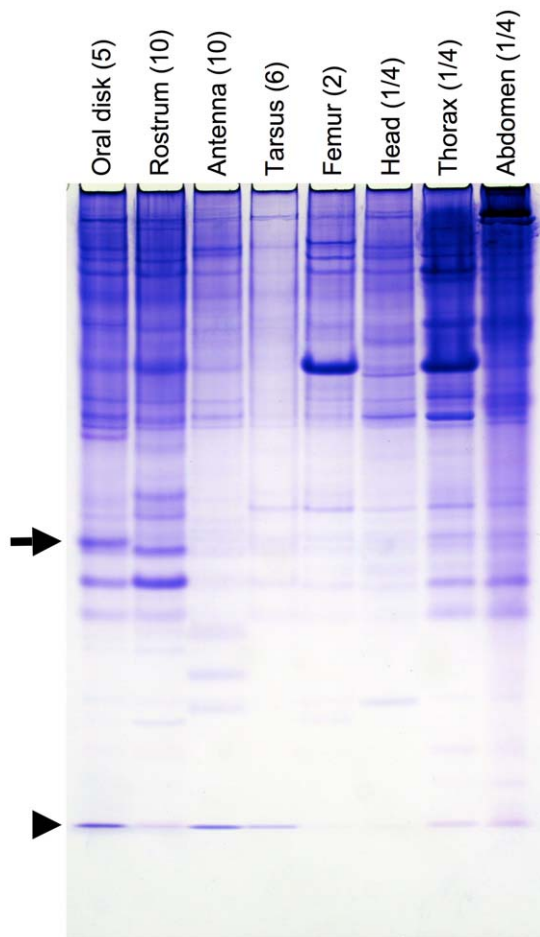
Figure 1. Identification of an oral disk-specific protein by native PAGE analysis. Protein was extracted from each experimental tissue of females at day 3 adult stage, separated by 15% native PAGE, and visualized with Coomassie Brilliant Blue-R250 staining. The source of the protein is shown at top of the gel profile. The number of individuals from which the tissues were collected is indicated in parenthesis. The arrow and arrowhead indicate the migration of an oral disk-specific protein and a chemical sense-related lipophilic ligand-binding protein (CRLBP), respectively. doi:10.1371/journal.pone.0051779.g001
