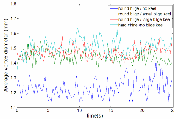
Figure 6. Temporal evolution of the average vortex diameter
