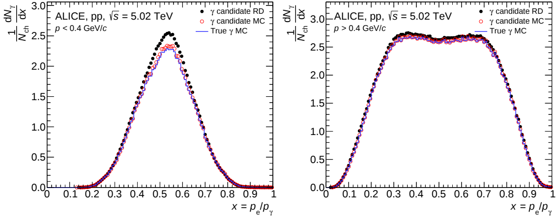
Figure 1. Distribution of the electron fractional energy ( x ) for photon candidates with p < 0.4 GeV/c (left) and with p > 0.4 GeV/c (right) reconstructed in real data (black points), in Monte Carlo simulations (red points), and for verified photons in MC simulations (blue lines) where PYTHIA8 is used as input event generator.
