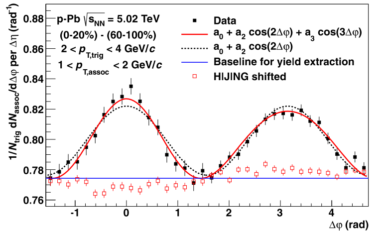
Fig. 3. Left: Associated yield per trigger particle in \Delta\phi and \Delta\eta for pairs of charged particles with 2 < p_{T,\text{trig}} < 4 \text{ GeV}/c and 1 < p_{T,\text{assoc}} < 2 \text{ GeV}/c in p-Pb collisions at \sqrt{s_{\text{NN}}} = 5.02 \text{ TeV} for the 0–20% multiplicity class, after subtraction of the associated yield obtained in the 60–100% event class. Top right: the associated per-trigger yield after subtraction (as shown on the left) projected onto \Delta\eta averaged over |\Delta\phi| < \pi/3 (black circles), |\Delta\phi - \pi| < \pi/3 (red squares), and the remaining area (blue triangles, \Delta\phi < -\pi/3 , \pi/3 < \Delta\phi < 2\pi/3 and \Delta\phi > 4\pi/3 ). Bottom right: as above but projected onto \Delta\phi averaged over 0.8 < |\Delta\eta| < 1.8 on the near side and |\Delta\eta| < 1.8 on the away side. Superimposed are fits containing a \cos(2\Delta\phi) shape alone (black dashed line) and a combination of \cos(2\Delta\phi) and \cos(3\Delta\phi) shapes (red solid line). The blue horizontal line shows the baseline obtained from the latter fit which is used for the yield calculation. Also shown for comparison is the subtracted associated yield when the same procedure is applied on HIJING shifted to the same baseline. The figure shows only statistical uncertainties. Systematic uncertainties are mostly correlated and affect the baseline. Uncorrelated uncertainties are less than 1%. (For interpretation of the references to colour in this figure legend, the reader is referred to the web version of this Letter.)
