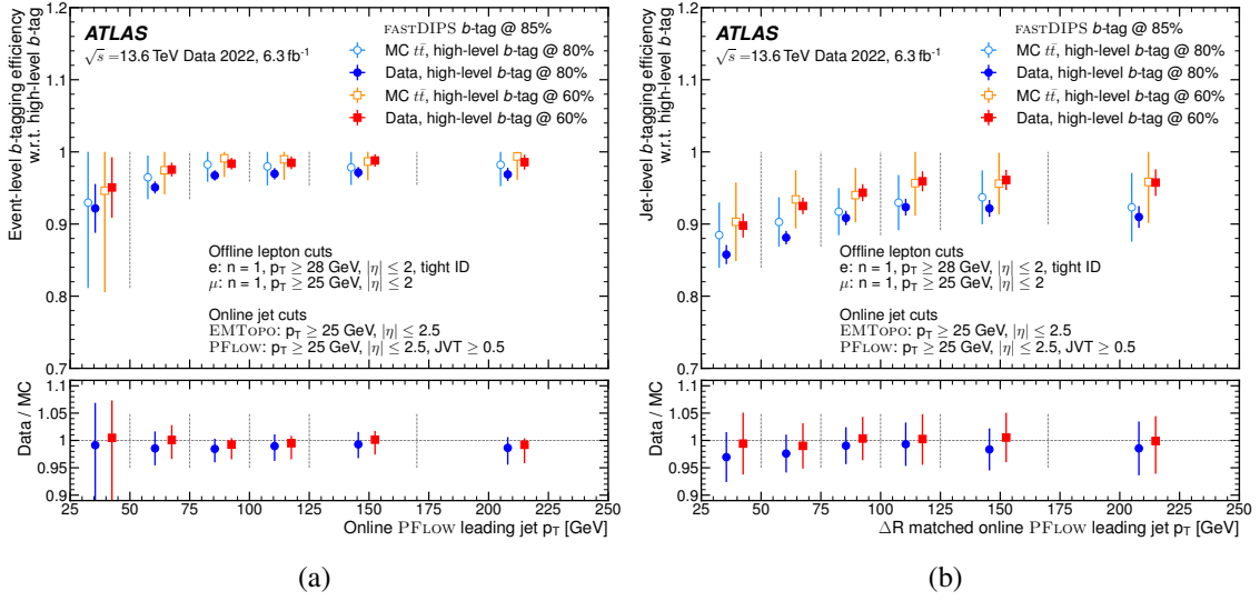
Figure 4. Event-level and jet-level efficiencies in simulated t\bar{t} events and data recorded by a trigger selecting t\bar{t} -like events, at \sqrt{s} = 13.6 \text{ TeV} . Figure (a) shows the event-level efficiency for at least one fast b -tag, in bins of the leading jet p_T , in events that already have at least one EMTopo jet and one high-level b -tag. Figure (b) shows the corresponding jet-level efficiency for the fast b -tagging algorithm with respect to the high-level b -tagging one. The two plots have the same binning, bin edges are displayed with the vertical dashed lines. For the jet-level efficiency, EMTopo and PFlow jets are geometrically matched with a \Delta R < 0.3 , and p_T relative difference less than 10%. In both figures, the displayed uncertainties are statistical only. In the ratio panels, the errors are propagated as the quadratic sum of the statistical uncertainties.
