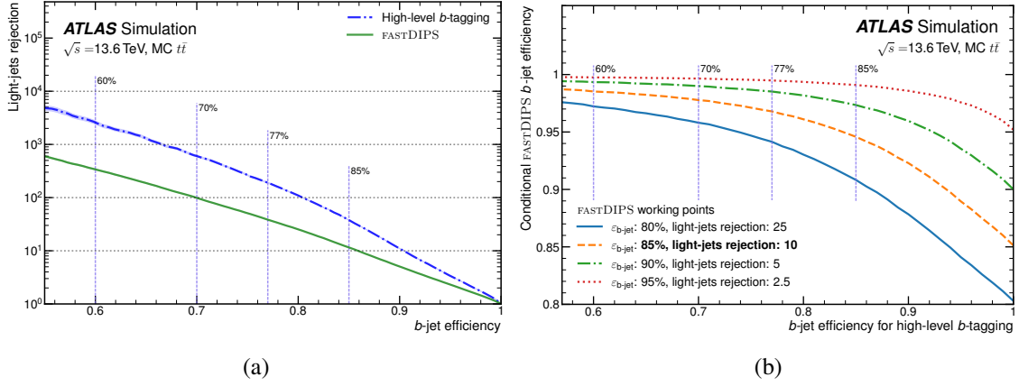
Figure 3. Comparisons of fast and high-level b -tagging. Fast b -tagging is applied to EMTopo jets, while high-level b -tagging is applied to PFlow jets. Figure (a) gives the light-jet rejection as a function of b -tagging efficiency for both approaches, fast and high-level b -tagging. Statistical uncertainties for each ROC curve, represented with shaded regions, are computed assuming binomial efficiency errors. Figure (b) gives the conditional efficiency for fast b -tagging to identify a true EMTopo b -jet, as a function of the efficiency of the high-level b -tagging selection on PFlow jets. The latter are matched with EMTopo jets. Jets are required to have p_T > 20 GeV. The different curves show the conditional efficiencies for multiple FASTDIPS discriminant selections. The working point with 85% efficiency is used in the trigger. The purple vertical dashed lines represent the most common working points used for b -tagging.
