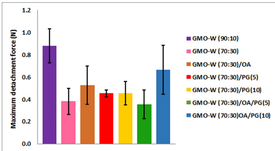
FIGURE 4 – Maximum detachment force ( F_{max} ) of liquid crystalline systems obtained using a Texture Analyser TA.XT Plus (Stable Micro Systems) and pig buccal cheek (n=3). Glyceryl monooleate (GMO), water (W), oleic acid (OA), propylene glycol at 5% (PG5), propylene glycol at 10% (PG10).
