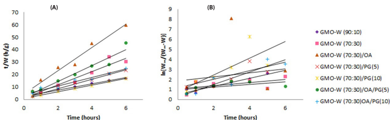
FIGURE 3 – Swelling isotherms of liquid crystalline systems according to: (A) the second-order kinetics (Equation 2) and (B) the first-order kinetics (Equation 1). Swelling data were obtained from Figure 1. W_{\infty} is the maximum water uptake, W is the water uptake at a time t , (W_{\infty}-W) is the unrealized water uptake (Schoot, 1992). Glyceryl monooleate (GMO), water (W), oleic acid (OA), propylene glycol at 5% (PG5), propylene glycol at 10% (PG10).
