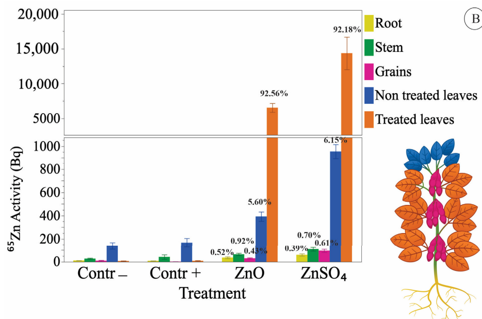
Figure 3. (A) ^{65}\text{Zn} activity in plant parts from the harvest after the first harvest (treatment in V4 and harvest V6–V8). (B) ^{65}\text{Zn} activity in plant parts from the harvest second harvest (treatment in V6–V8 and harvest R5.3–R5.4). Contr– is the plants cultivated in solution with 10% of Zn recommendation and no leaf application, and Contr+ is plants cultivated in solution with 100% of Zn recommendation and no leaf application. The bars indicate the standard error of the mean. The coefficient of variation is represented as CV%. Zn applied on the plant leaves was translocated to other plant parts. Values in % represent the activity of Zn in each part of the plant relative to the total activity across all parts of the plant.
