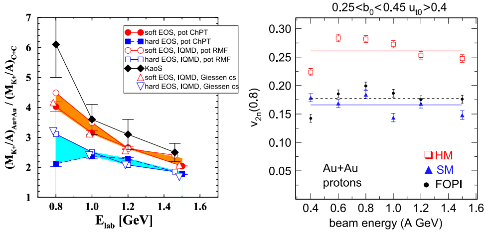
Fig. 3.2. Left panel: Beam energy dependence of K^+ yield ratios in inclusive Au + Au collisions and C + C collisions between E_{kin} = 0.8 – 1.5 AGeV ( \sqrt{s_{NN}} = 2.24 – 2.52 GeV). A comparison of RQMD [172] and IQMD [445] model calculations indicates a soft EOS ( K_0 = 200 MeV, red symbols) instead of a hard EOS ( K_0 = 380 MeV, blue symbols) when compared to KaoS data [444] (black symbols). Source: Figure from [442]. Right panel: Beam-energy dependence of the elliptic flow for protons in Au + Au collisions at E_{kin} = 0.4 AGeV ( \sqrt{s_{NN}} = 2.07 GeV) (black symbols) as measured by the FOPI experiment [176]. Comparison to IQMD transport calculations with momentum dependence prefers a soft EOS (blue triangles) over a hard EOS (red squares), yielding K_0 = 190 \pm 30 MeV. Source: Figure from [60].
