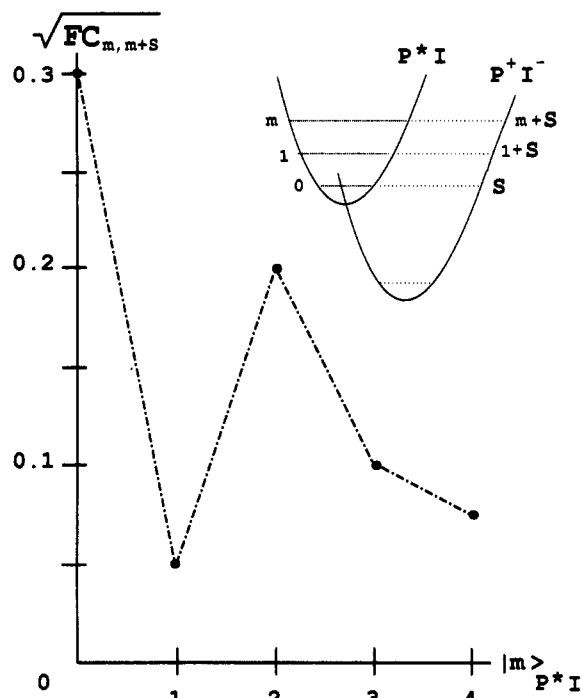
Figure 9. Plot of the square root of the Franck-Condon factor between any initial |m\rangle_{P+I} vibronic state and any final |m+S\rangle_{P+I-} state. The primary transfer is assumed to be activationless with S = 30 .
