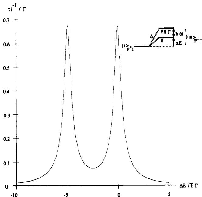
Figure 6. Behavior of the decay rate of |i\rangle_{P+I} as it moves from resonance to off resonance with respect to |n\rangle_{P+I} . The values of \Delta/\hbar\Gamma and \hbar\omega/\hbar\Gamma are chosen in different rate regimes (see Figure 5). Here, \Delta/\hbar\Gamma = 0.5 , \hbar\omega/\hbar\Gamma = 5 .
