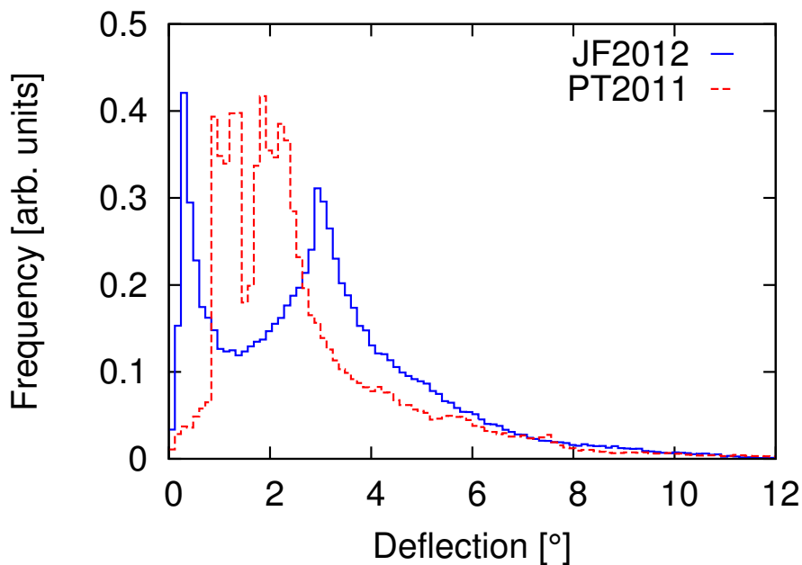
Figure 3. Distribution of UHECR deflections in two Galactic magnetic field models marked PT2011 [44] and JF2012 [45] for the regular component. The energies of actual UHECRs are renormalized to show the distributions for E/Z = 100 EeV. The double-peak structure is mostly due to the fact that UHECRs from different Galactic hemispheres undergo different deflections.
