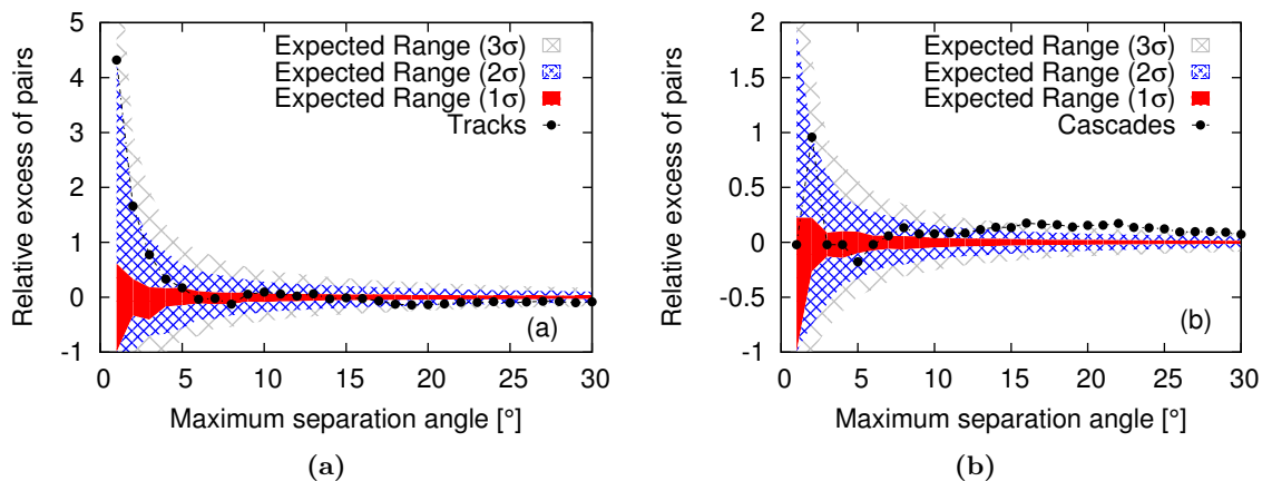
Figure 6. Relative excess of pairs, [n_p(\alpha)/\langle n_p^{\text{iso}}(\alpha) \rangle] - 1 , as a function of the maximum angular separation between the neutrino and UHECR pairs, for the analysis done with the track-like events (a) and with the cascade events (b). The 1\sigma , 2\sigma and 3\sigma fluctuations expected from an isotropic distribution of arrival directions of CRs are shown in red, blue and grey, respectively.
