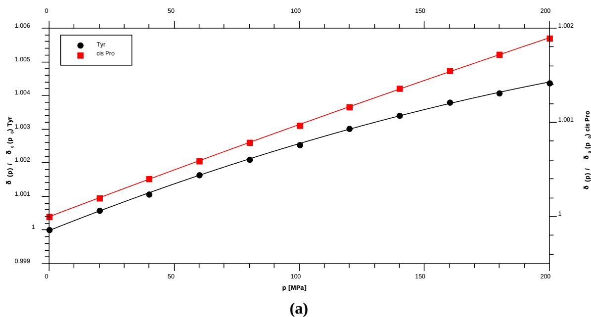
Figure 3. Pressure dependent ^{15}\text{N} chemical shift changes of selected residues. The chemical shifts \delta are plotted as a function of pressure p for some residues X. For a better comparison the inverse of the initial value at ambient pressure was used as normalization factor for each data series. (a) Non-linearity of the pressure dependence of cis-proline and tyrosine residues. (b) The pressure dependence of chemical shifts of selected residues.
