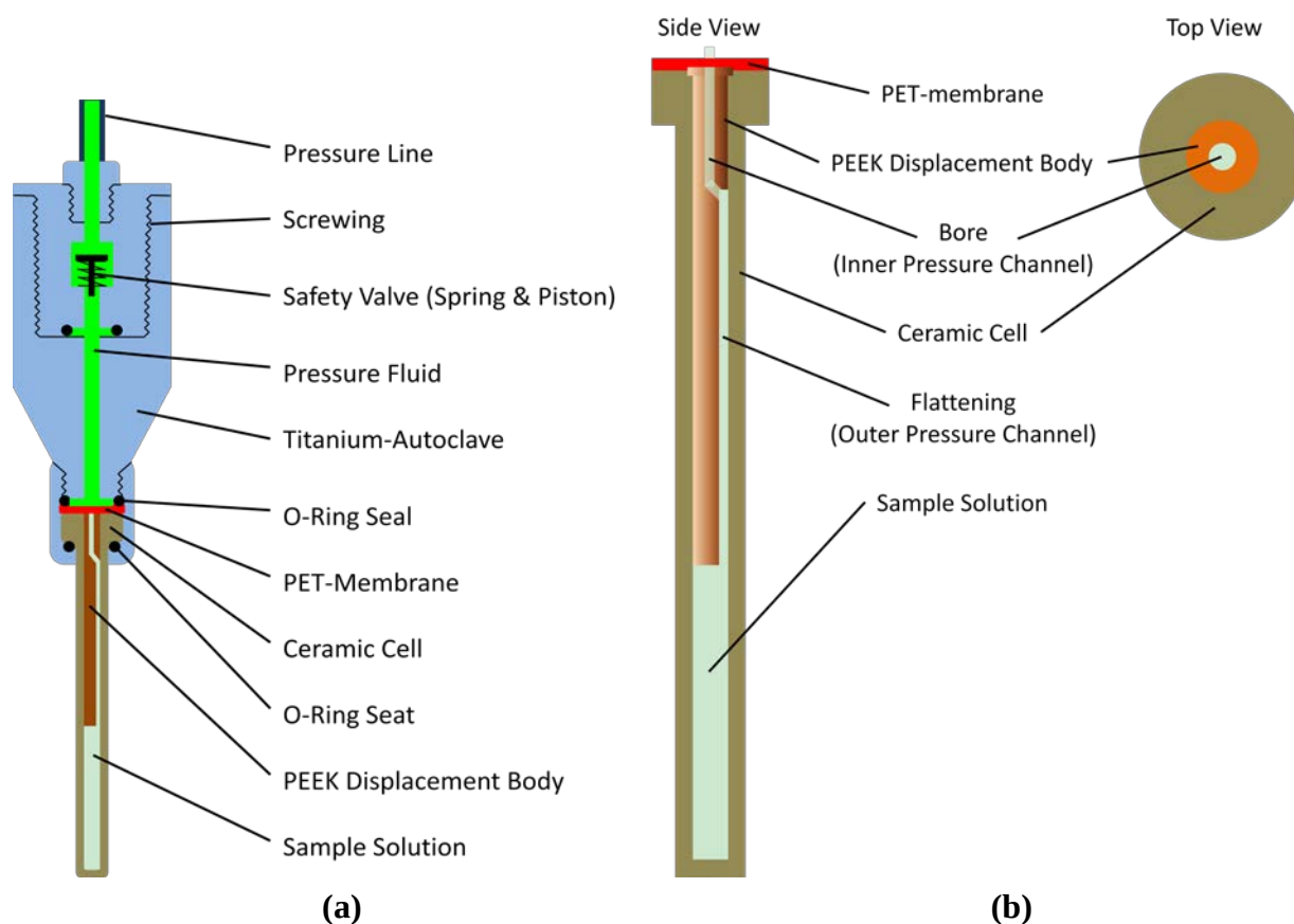
Figure 6. High pressure autoclave. (a) The high pressure autoclave holding the ceramic cell is similar to that provided by Daedalus Corporation [14], but has additionally a safety valve analogous to that described earlier by Beck Erlach et al. [15]; (b) A PET membrane was posed on top of the ceramic cell, and a bored and flattened cylindrical displacement body was inserted into the tube.
