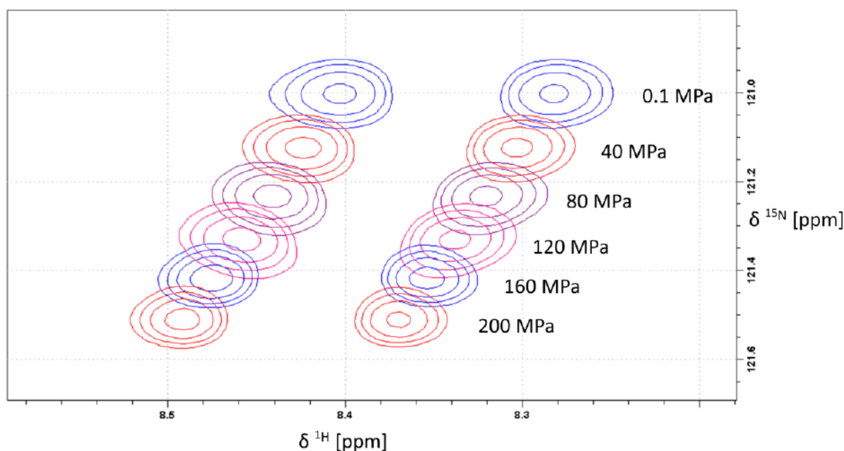
Figure 1. Pressure dependent ^1\text{H} - ^{15}\text{N} -HSQC spectra of backbone amide region of arginine. The samples contained 5 mM Ac-Gly-Gly-Arg-Ala-NH 2 in 20 mM Tris-HCl in 90% H 2 O/10% D 2 O, pH 6.7. Measurements were performed at 283 K. Data processing was done with Gaussian filter in both directions using negative line broadenings of -10 Hz and -3 Hz for ^{15}\text{N} and ^1\text{H} , respectively.
