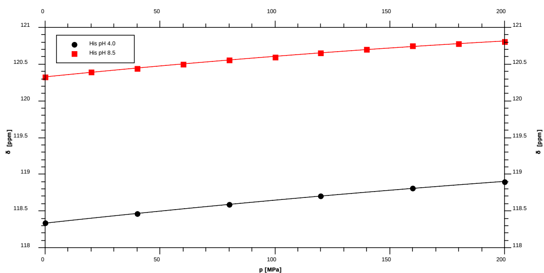
Figure 4. Pressure dependence of backbone ^{15}\text{N} chemical shift resonances of histidine Ac-Gly-Gly-His-Ala- \text{NH}_2 . Sample composition, experimental conditions and data fitting are described in Table 1. The sample was measured at pH 4.0 and pH 8.5.
