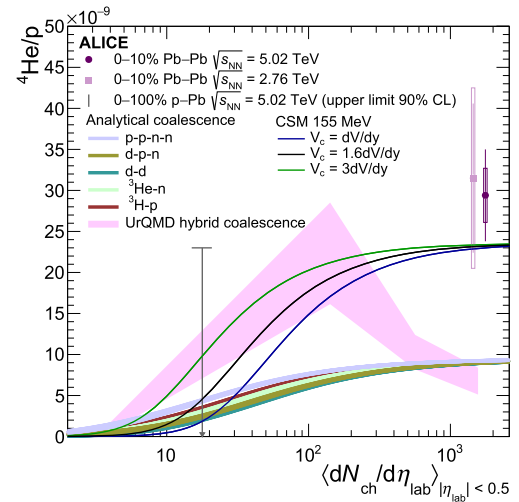
Fig. 5. ^4\text{He}/p ratios for the measured data points as a function of charged-particle multiplicity \langle dN_{\text{ch}}/d\eta \rangle_{|\eta_{\text{lab}}| < 0.5} compared to model predictions. For comparison the result from the 10% most central Pb–Pb collisions at \sqrt{s_{\text{NN}}} = 2.76 TeV [42] and the upper limit at 90% CL from p–Pb collisions at \sqrt{s_{\text{NN}}} = 5.02 TeV [126] is also shown. The thermal model curves are from the CSM [63]. For the coalescence model two different approaches are displayed: analytical and UrQMD hybrid coalescence [127,128]. The analytical coalescence is shown for five different substructures and the thickness of the bands reflects the uncertainties of the calculation. For the UrQMD model the band is representing the statistical uncertainty of the prediction.
