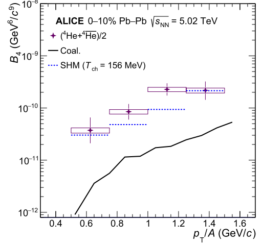
Fig. 4. The coalescence parameter B_4 as a function of p_T/A , calculated from the averaged ^4\text{He} and ^4\overline{\text{He}} spectra and the protons from [116]. Statistical uncertainties are indicated by the vertical lines and the boxes correspond to the systematic uncertainties. The blue dashed line and the full black line indicate the values for the SHM combined with blast-wave p_T shapes and the coalescence predictions from Refs. [91,92], respectively.
