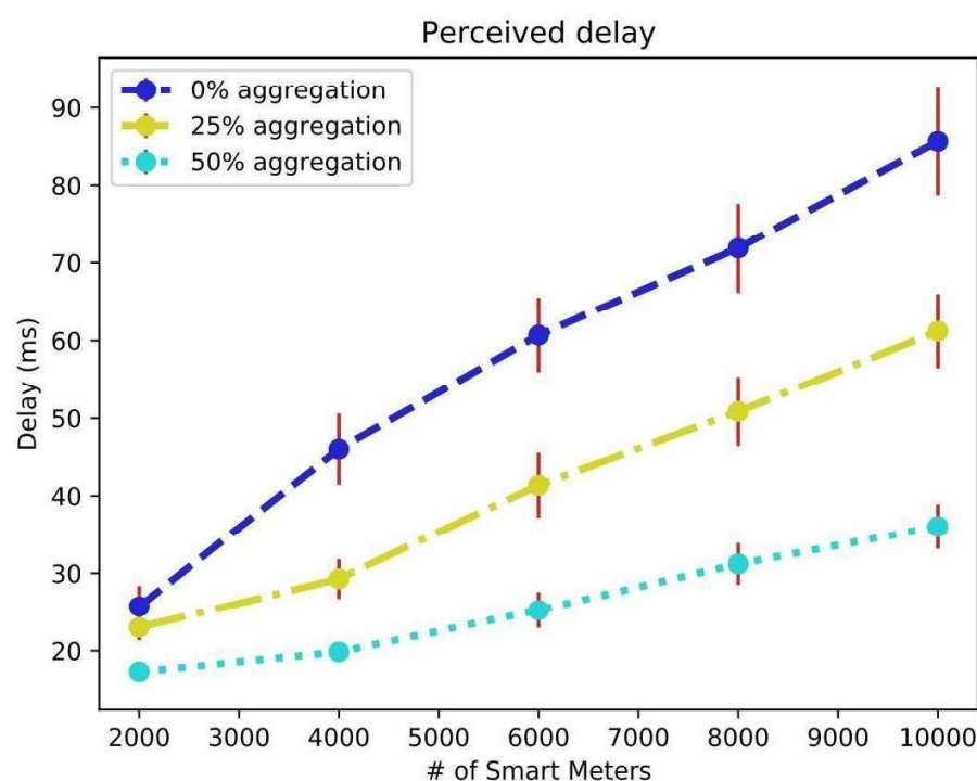
Figure 6. Average message delay (in milliseconds) sent from multiple smart meters to MEC server in simulation of 0%, 25%, and 50% aggregation.
