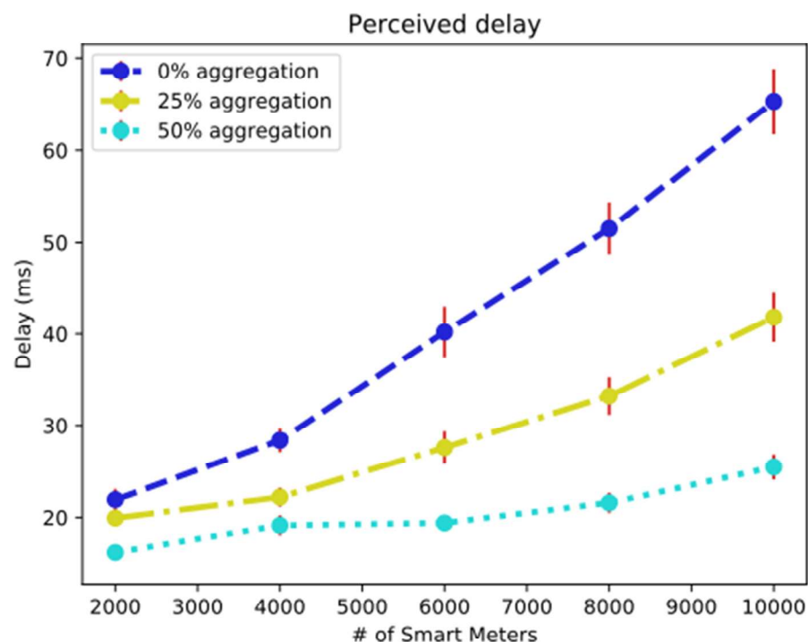
Figure 8. Average message delay after the relocation of ERB 3.
