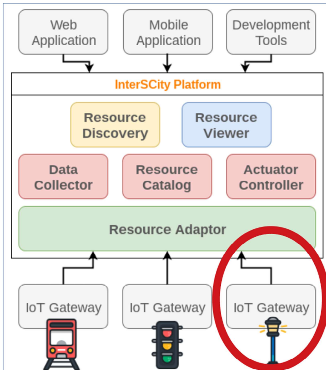
Figure 3. InterSCity is a web-based microservice. IoT gateway for SPG is emphasized in the red ellipse.
