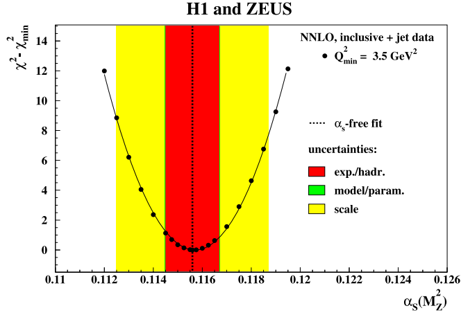
Figure 18. Distribution of \Delta\chi^2 = \chi^2 - \chi_{\min}^2 versus \alpha_S(m_Z^2) for HERAPDF2.0NN-LOJets fits with fixed \alpha_S(m_Z^2) values. Experimental, model/parametrization, and scale uncertainties are illustrated (figure from [243]).
