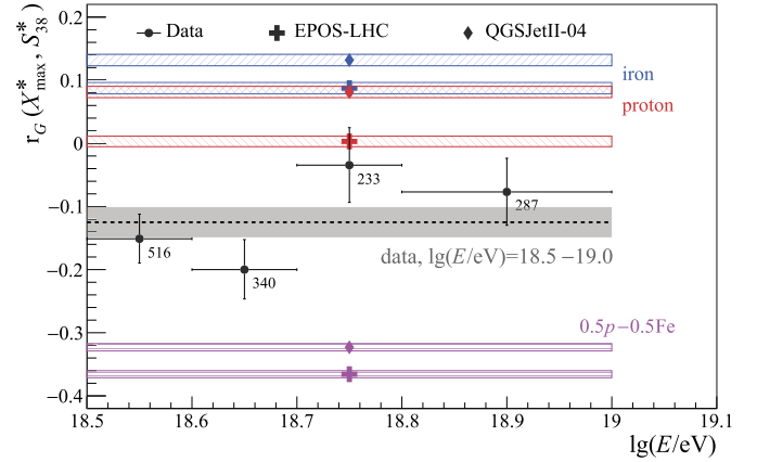
Fig. 3. The correlation coefficients r_G for data in the energy bins \lg(E/\text{eV}) = 18.5\text{--}18.6 ; 18.6\text{--}18.7 ; 18.7\text{--}18.8 ; 18.8\text{--}19.0 . Numbers of events in each bin are given next to the data points. The gray band shows the measured value for data in the whole range \lg(E/\text{eV}) = 18.5\text{--}19.0 . Predictions for the correlations r_G in this range for pure proton and iron compositions, and for the extreme mix 0.5p-0.5\text{Fe} from EPOS-LHC and QGSJetII-04 are shown as hatched bands (for Sibyll 2.1 values are similar to those of QGSJetII-04). The widths of the bands correspond to statistical errors.
