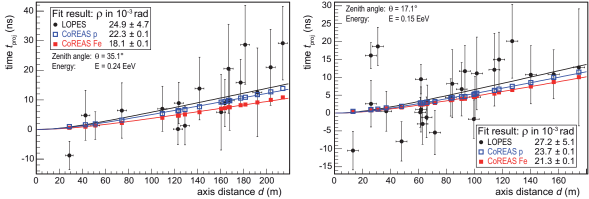
Figure 5. Two example events: arrival times and fitted hyperbolic wavefront (equation (2.2) for b fixed to -3 ns) for the LOPES measurements and CoREAS simulations for protons and iron nuclei as primary particles; the measured and simulated arrival times (= time of the maximum) are corrected for the expected arrival time of an ideal plane wavefront, which would correspond to a horizontal line at 0 ns. Since the simulations are affected by shower-to-shower fluctuations, it is not expected that they would agree exactly with the measurements for individual events, but only on average. The x-error bars of the measurements are due to the uncertainty of the shower axis which is dominated by the core uncertainty; the y-error bars are dominated by the uncertainty due to noise, and include also the small calibration uncertainty.
