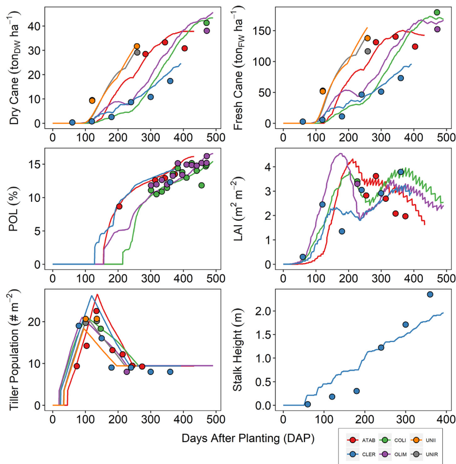
Fig. 6. Comparison of simulated (lines) and observed (circles) dry and fresh cane biomass (ton ha -1 ), sucrose content (POL, %), leaf area index (LAI, m 2 m -2 ), tiller population (# m -2 ) and stalk heights (m) across different Brazilian regions. Code IDs for each site are provided in Table 2.
