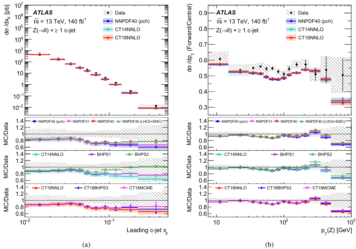
Fig. 14 Measured fiducial cross-section for Z + \geq 1 c -jet production as a function of a leading c -jet x_F and b R(p_T(Z)) . The data are compared with the nominal MGMC+PY8 FxFx predictions and with those using the PDFs testing several IC models. The error bars corre-
