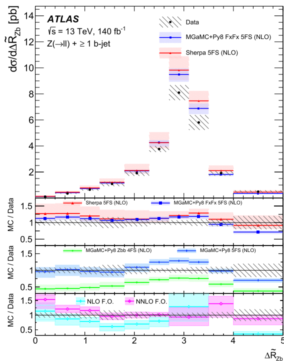
Fig. 10 Measured fiducial cross-section for Z + \geq 1 b -jet production as a function of \Delta R_{Zb} . The data are compared with the predictions from the 5FS multi-leg generators MGaMC+Py8 FxFx and SHERPA 2.2.11, with MGaMC+Py8 4FS (NLO) and MGaMC+Py8 5FS (NLO), and with NLO and NNLO fixed-order (F.O.) predictions [3]. The error bars correspond to the statistical uncertainty, and the hatched bands to the data statistical and systematic uncertainties added in quadrature. The shaded bands correspond to the statistical and theoretical uncertainties of the predictions added in quadrature. For the fixed-order predictions, the uncertainties in the hadronisation and MPI and flavour definition algorithm corrections are also added in quadrature to the total, while pure theory uncertainty of the predictions are shown as the range between the horizontal lines
