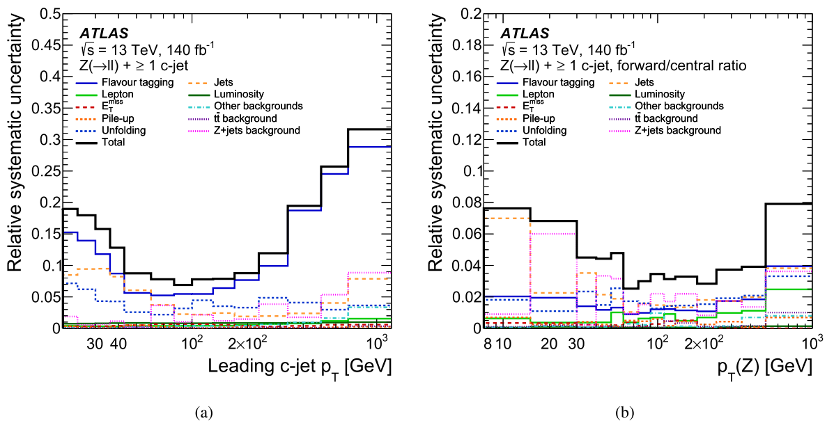
Fig. 6 Relative systematic uncertainties in a the fiducial cross-section as a function of leading c -jet p_T ( p_{T,c}^0 ) and b the ratio of the cross-sections as functions of Z boson p_T in forward and central Z boson
