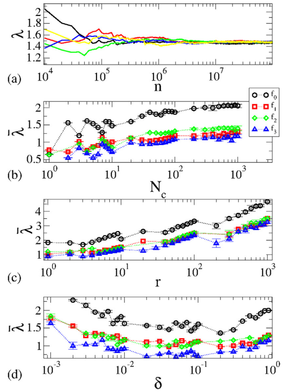
Fig. 4. (Colour online.) (a) Plot of the Lyapunov exponent as a function of n for five different initial conditions and considering the function f_0 . The parameters used were N_c = 10 , r = 1 and \delta = 0.5 . For the functions f_0 , f_1 , f_2 and f_3 we have: (b) \bar{\lambda} vs N_c for fixed r = 1 and \delta = 0.5 ; (c) \bar{\lambda} vs r for fixed N_c = 33.18 and \delta = 0.5 ; (d) \bar{\lambda} vs \delta for fixed N_c = 33.18 and r = 1 .
