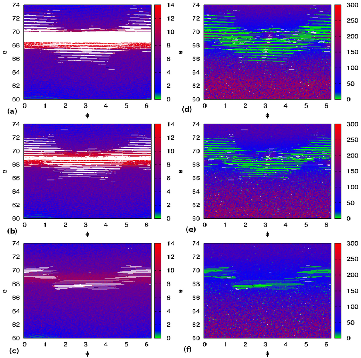
Fig. 8. (Colour online.) Grid of different initial conditions (\phi_0, e_0) showing in colour the logarithm of the escape time (LET) for: (a) r = 80 ; (b) r = 100 ; (c) r = 200 . Number of different return times (NDRT) for: (d) r = 80 ; (e) r = 100 ; (f) r = 200 . The escape windows are situated at e_1 < 59 and e_1 > 75 . The function F_0 was used to obtain the results.
