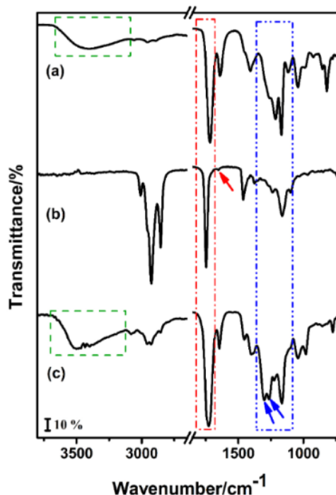
Figure 2. MIR spectra of precursors a) PP, b) PFVO1, and c) the polymer PPF1
