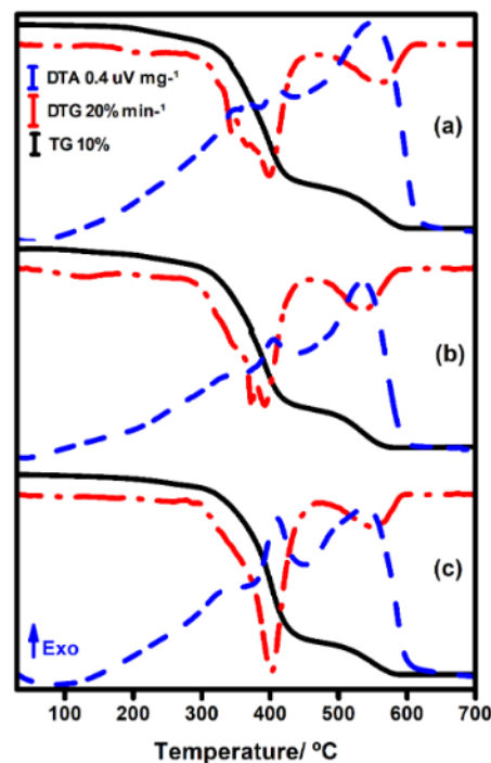
Figure 6. TG/DTG-DTA curves of polymers obtained from different passion fruit vegetable oils: a) PPVO1, b) PPVO2, and c) PPVO3
