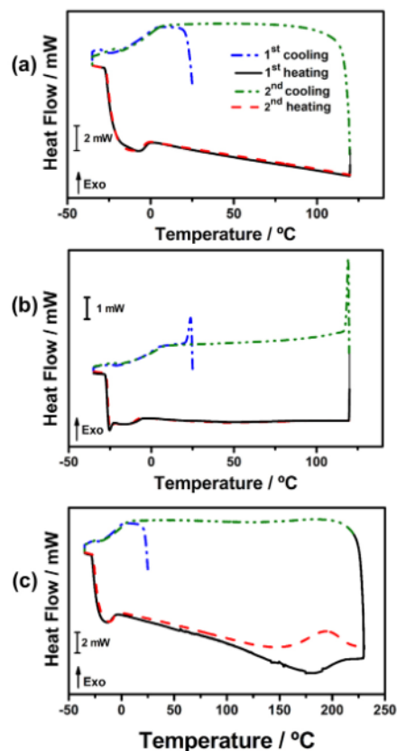
Figure 7. DSC curves of a) PFVO1, b) PFVO2, and c) PFVO3
