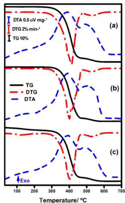
Figure 5. TG/DTG-DTA curves of different passion fruit vegetable oils: a) PFVO1, b) PFVO2, and c) PFVO3
