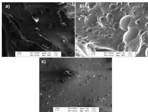
Figure 9. SEM images of a) PPF1, b) PPF2, and c) PPF3
