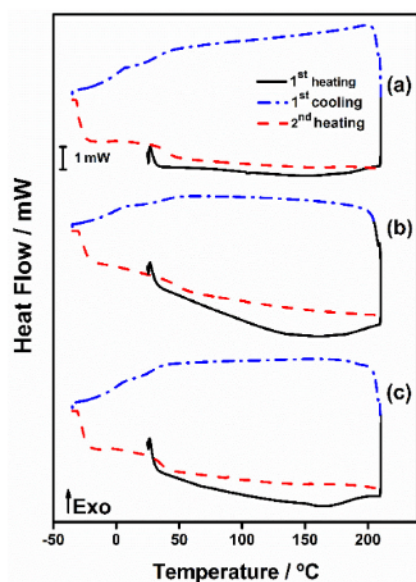
Figure 8. DSC curves of polymers a) PPF1, b) PPF2, and c) PPF3
