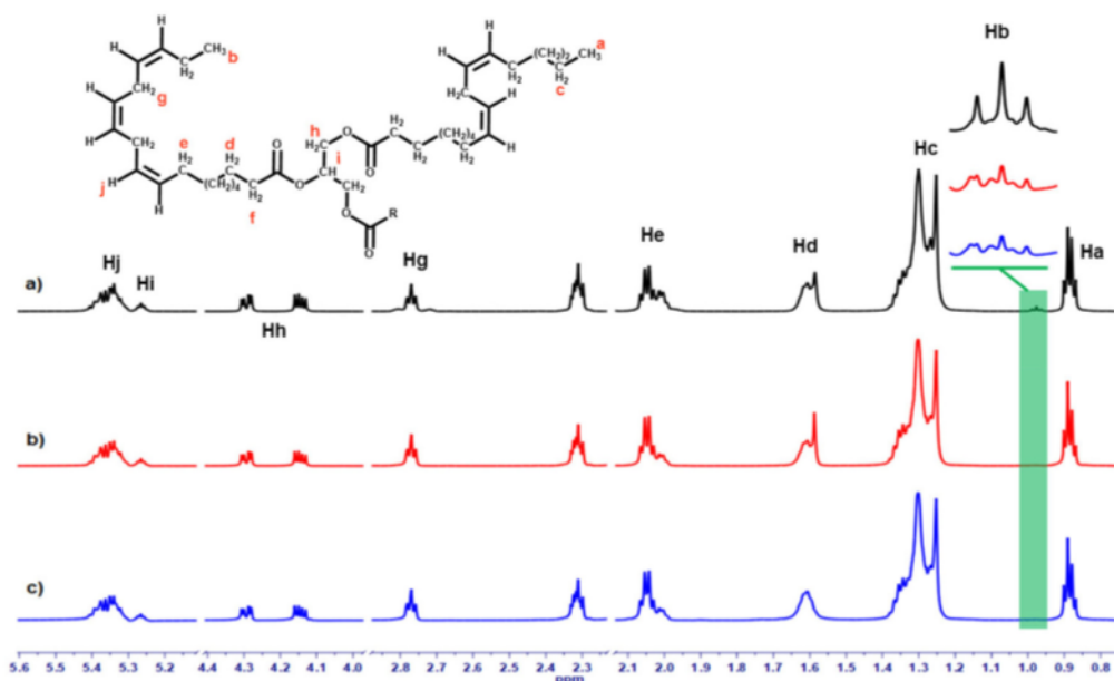
Figure 3. ^1\text{H} -NMR spectra (600 MHz, \text{CDCl}_3 ) of different passion fruit vegetable oils: a) PFVO1, b) PFVO2, and c) PFVO3, representative structure of a triglyceride and its respective protons
