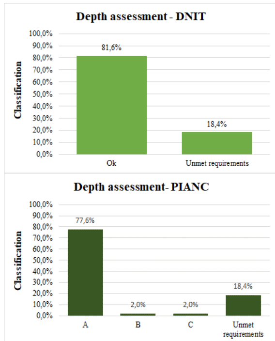
Figure 5. Verification of sections regarding depth criteria.
