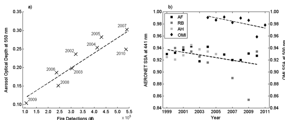
Figure 1. (a) Scatter plot of total fire detections and average AOD over the study domain and period. (b) (Square shapes) Aug–Oct averaged SSA derived from AERONET data for sites in the arc of deforestation: Alta Floresta (AF), Rio Branco (RB) and Abracos Hill (AH) between 1999 and 2010. (Diamond shapes) average Aug–Oct OMI SSA averaged over the study domain and period between 2004 and 2011. The difference in magnitude between OMI and AERONET may be due to the fact that OMI calculates SSA from retrievals at 388 nm, scaled to 500 nm, whereas AERONET calculates SSA from retrievals at 441 nm. Dashed lines in (a) and (b) show least-squares linear fits to the data.
