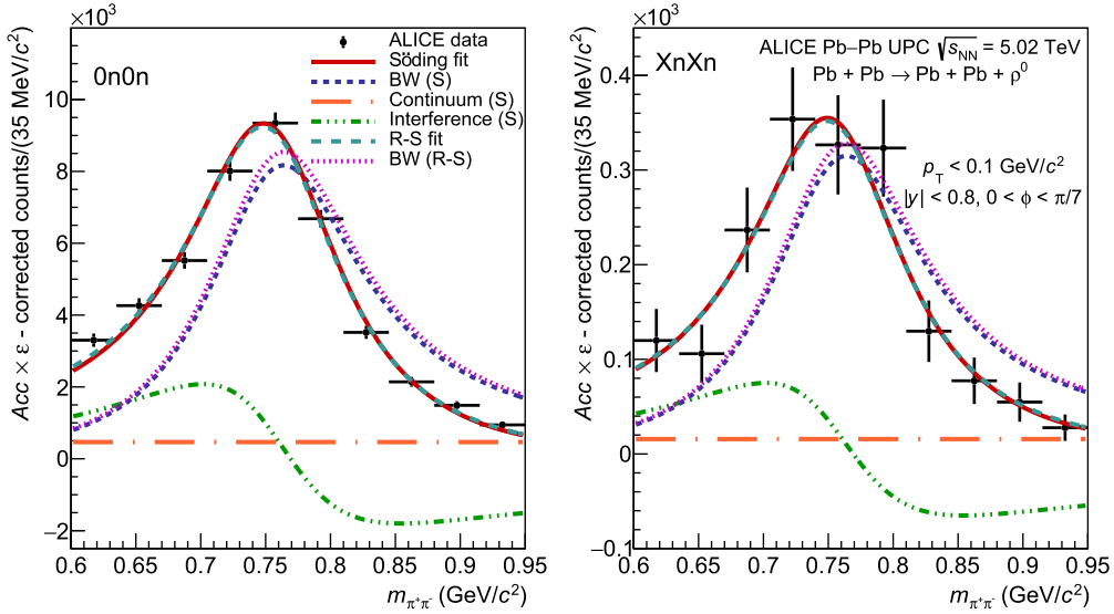
Fig. 1. Invariant-mass distribution of pion pairs, with superimposed Söding (solid line) and Ross-Stodolsky (dotted line) fits, for the range 0 < \phi < \pi/7 in the 0n0n (left) and XnXn (right) neutron classes. The different components of the pion-pair production amplitude in the Söding model are shown: the Breit-Wigner shape that describes the \rho^0 (finer dotted line), the continuum process (dash-dotted line), and the interference between the \rho^0 and the continuum (dash-dot-dot-dot line). The Breit-Wigner extracted from the Ross-Stodolsky model (finest dotted line) is also shown. In this example, the background contribution from misidentified muons is fixed to zero in the fit.
