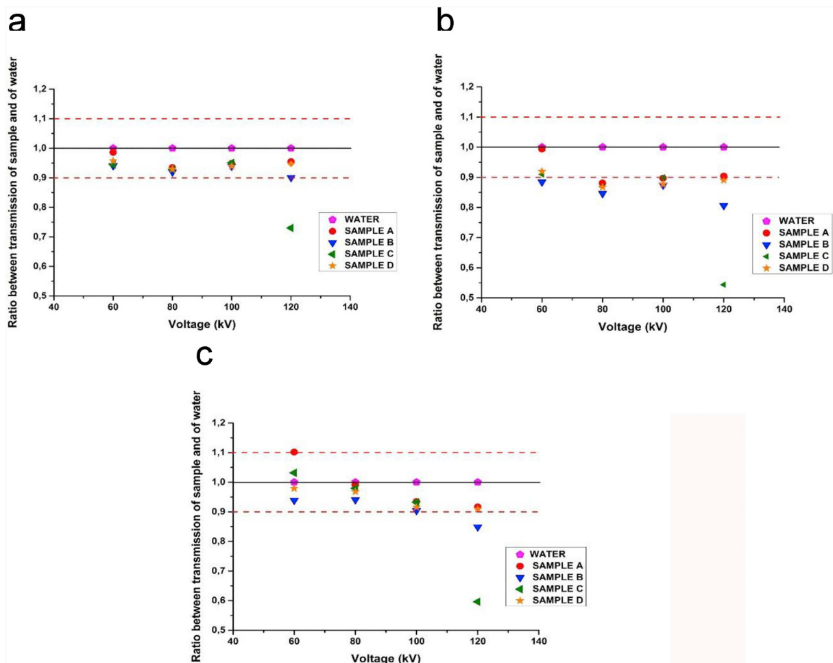
Fig. 5. Comparison between the transmissions of the samples and water for values of thicknesses of (a) 10 mm, (b) 30 mm and (c) 60 mm. Red dashed lines represent the range of \pm 10\% . (For interpretation of the references to colour in this figure legend, the reader is referred to the Web version of this article.)
